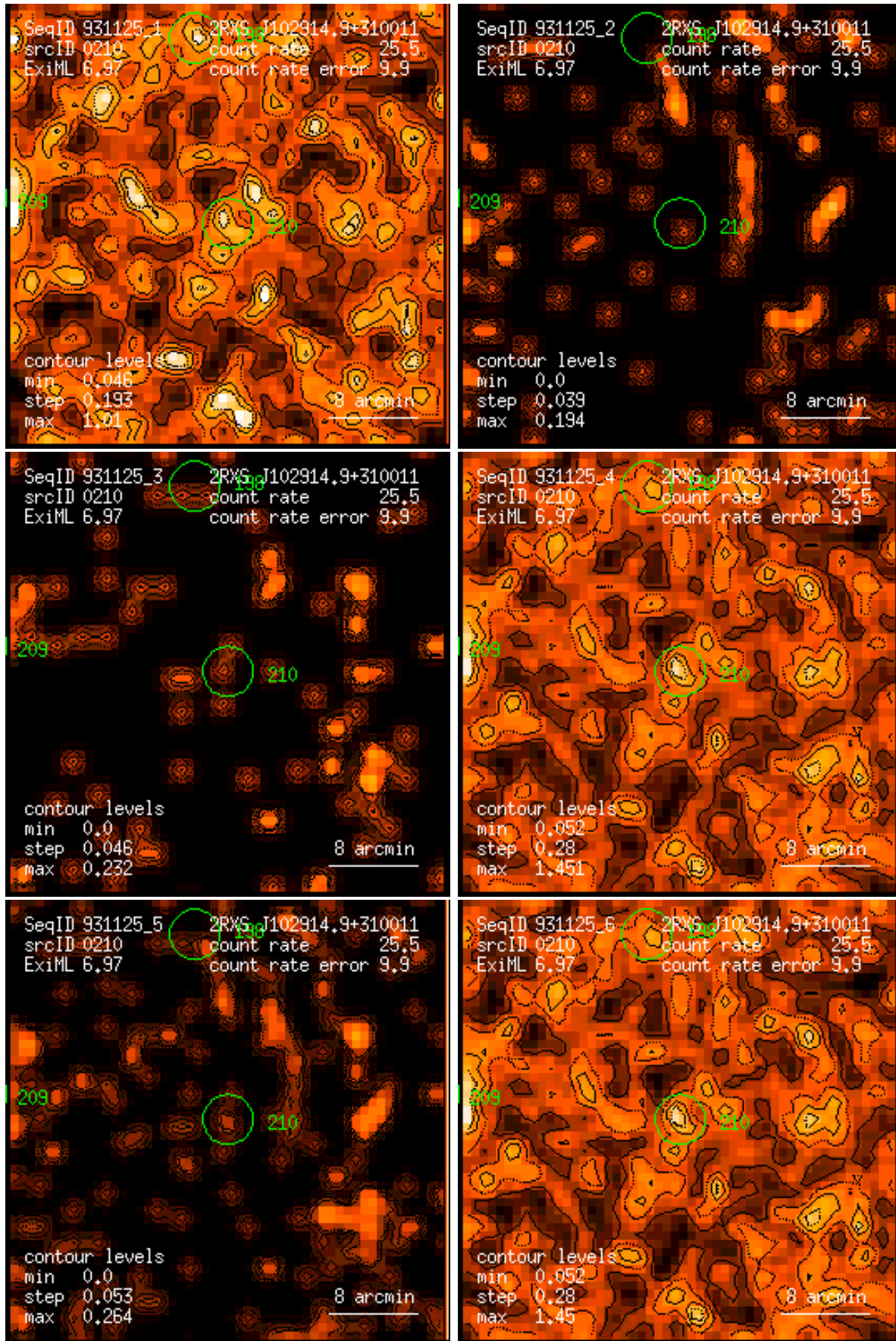
Figure 210: RASS 931125: detection 0210: band rate images, Gaussian filter: (1) PSPC channels 11 – 41, (2) 52 – 90, (3) 91 – 201, (4) 11 – 235, (5) 52 – 201, (6) 11 – 201. Broad band rates in counts/ks. Band rate contour levels in counts/ks/arcmin 2 .
