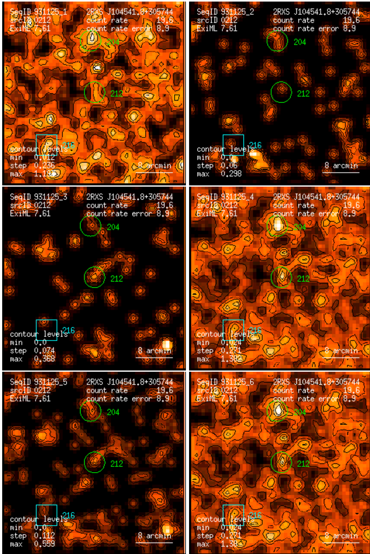
Figure 212: RASS 931125: detection 0212: band rate images, Gaussian filter: (1) PSPC channels 11 – 41, (2) 52 – 90, (3) 91 – 201, (4) 11 – 235, (5) 52 – 201, (6) 11 – 201. Broad band rates in counts/ks. Band rate contour levels in counts/ks/arcmin 2 .
