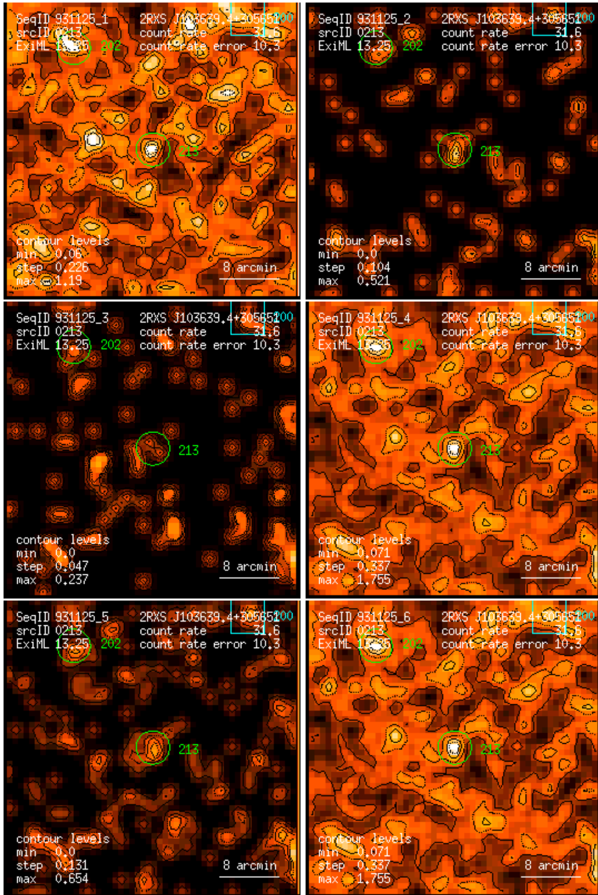
Figure 213: RASS 931125: detection 0213: band rate images, Gaussian filter: (1) PSPC channels 11 – 41, (2) 52 – 90, (3) 91 – 201, (4) 11 – 235, (5) 52 – 201, (6) 11 – 201. Broad band rates in counts/ks. Band rate contour levels in counts/ks/arcmin 2 .
