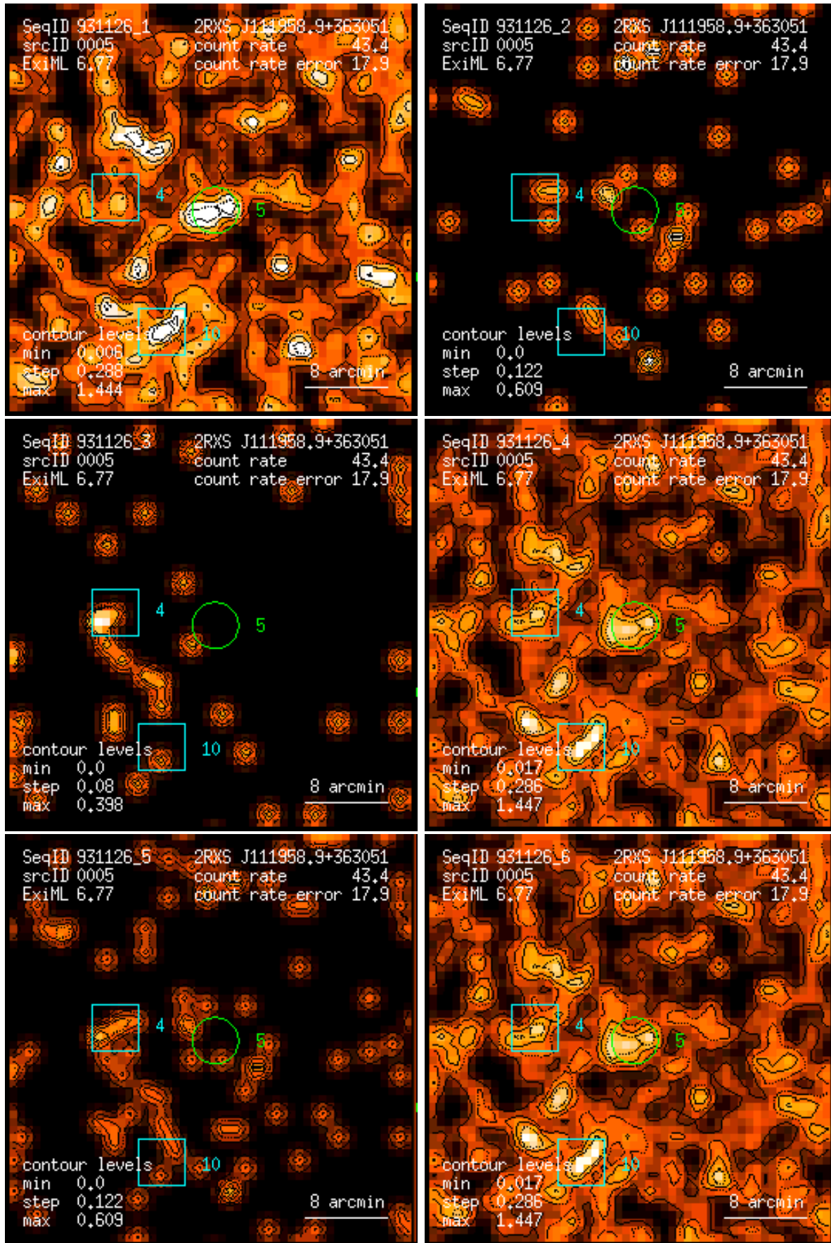
Figure 5: RASS 931126: detection 0005: band rate images, Gaussian filter: (1) PSPC channels 11 – 41, (2) 52 – 90, (3) 91 – 201, (4) 11 – 235, (5) 52 – 201, (6) 11 – 201. Broad band rates in counts/ks. Band rate contour levels in counts/ks/arcmin 2 .
