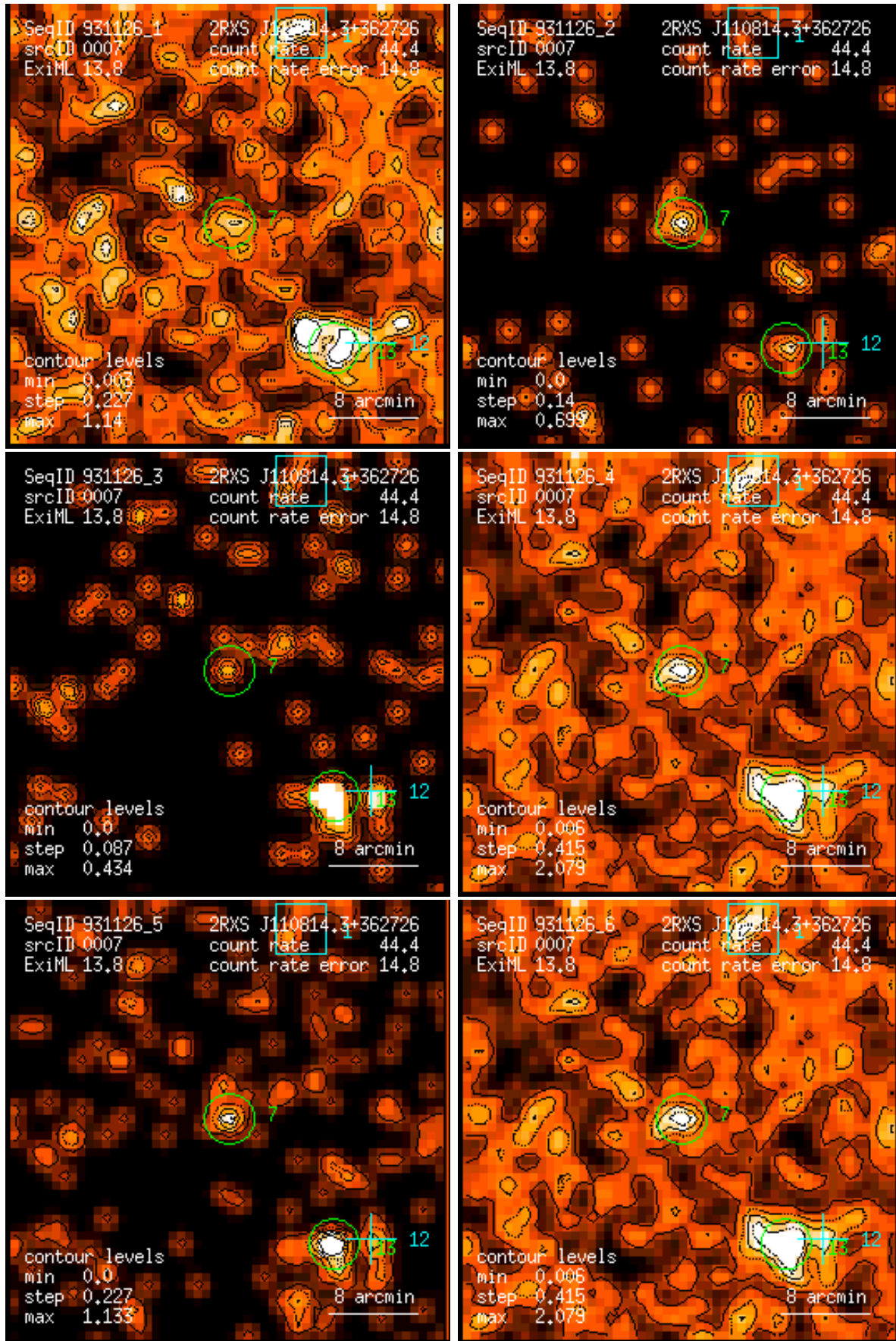
Figure 7: RASS 931126: detection 0007: band rate images, Gaussian filter: (1) PSPC channels 11 – 41, (2) 52 – 90, (3) 91 – 201, (4) 11 – 235, (5) 52 – 201, (6) 11 – 201. Broad band rates in counts/ks. Band rate contour levels in counts/ks/arcmin 2 .
