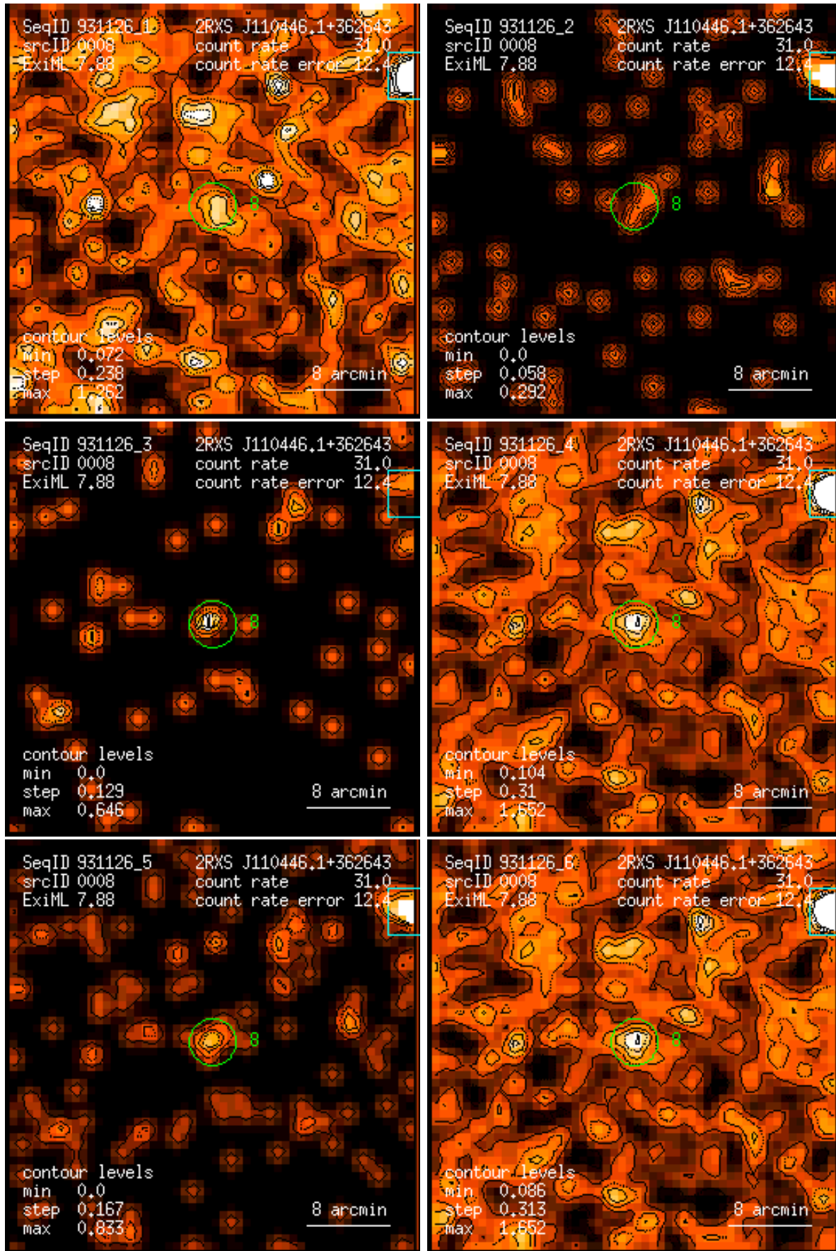
Figure 8: RASS 931126: detection 0008: band rate images, Gaussian filter: (1) PSPC channels 11 – 41, (2) 52 – 90, (3) 91 – 201, (4) 11 – 235, (5) 52 – 201, (6) 11 – 201. Broad band rates in counts/ks. Band rate contour levels in counts/ks/arcmin 2 .
