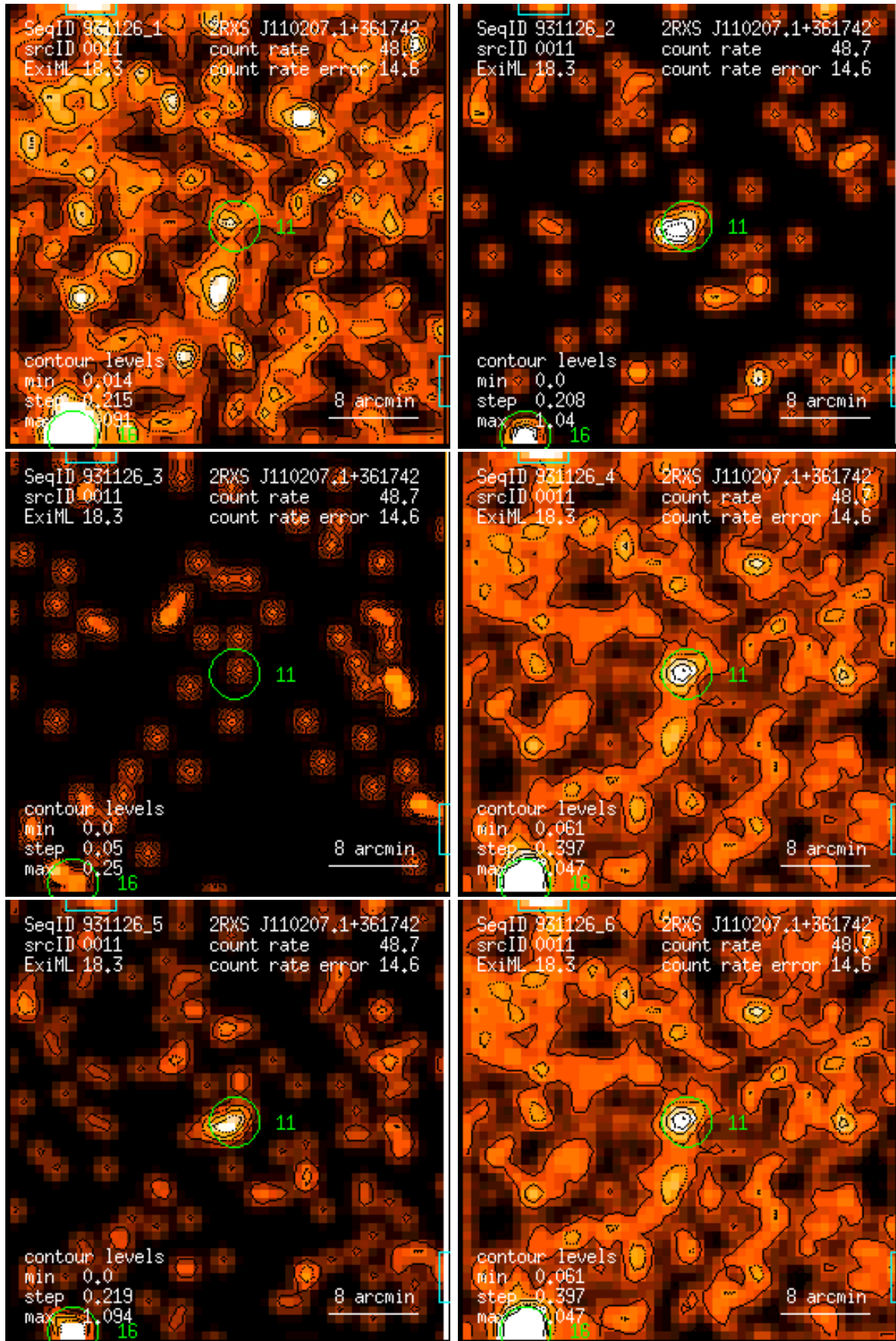
Figure 11: RASS 931126: detection 0011: band rate images, Gaussian filter: (1) PSPC channels 11 – 41, (2) 52 – 90, (3) 91 – 201, (4) 11 – 235, (5) 52 – 201, (6) 11 – 201. Broad band rates in counts/ks. Band rate contour levels in counts/ks/arcmin 2 .
