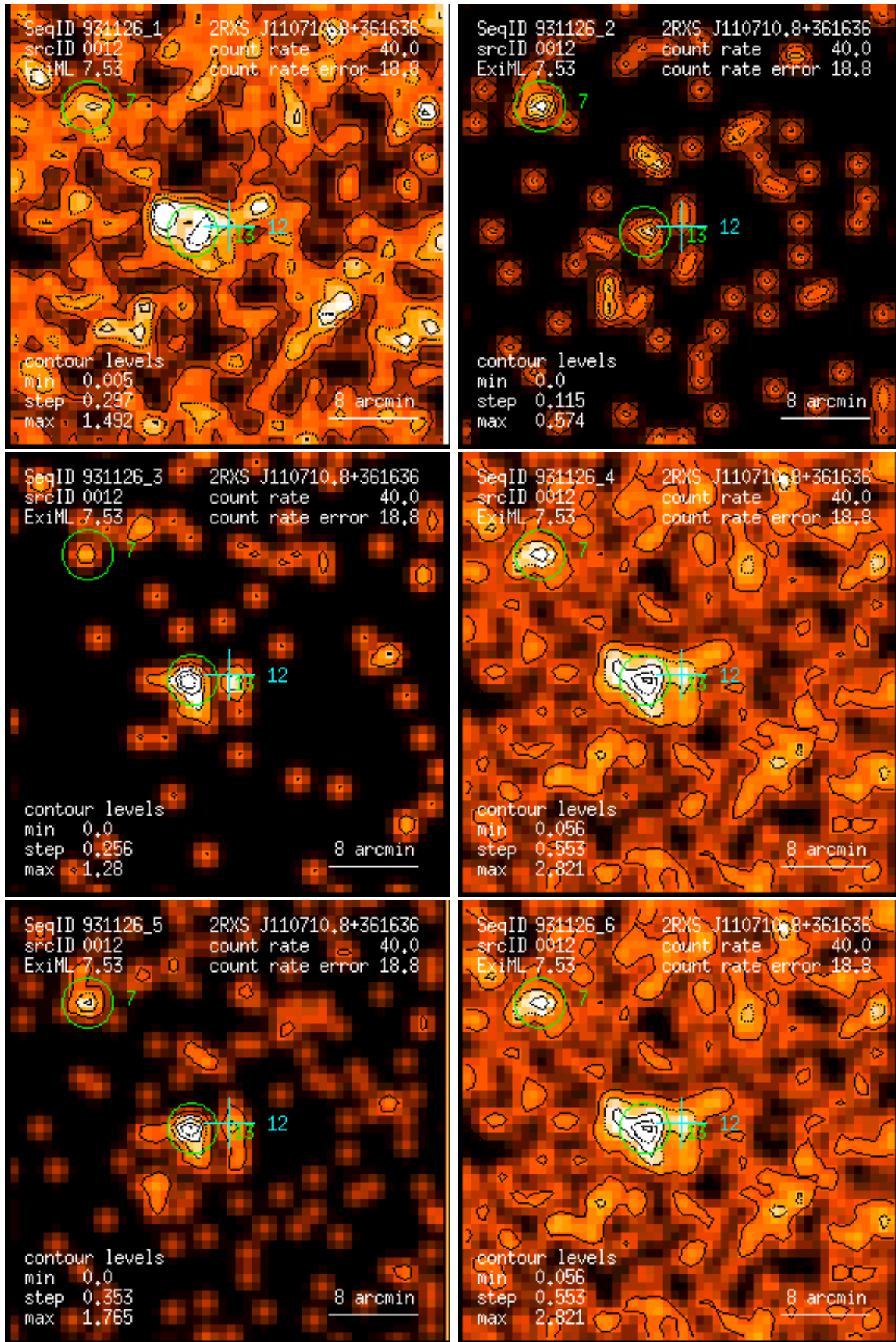
Figure 12: RASS 931126: detection 0012: band rate images, Gaussian filter: (1) PSPC channels 11 – 41, (2) 52 – 90, (3) 91 – 201, (4) 11 – 235, (5) 52 – 201, (6) 11 – 201. Broad band rates in counts/ks. Band rate contour levels in counts/ks/arcmin 2 .
