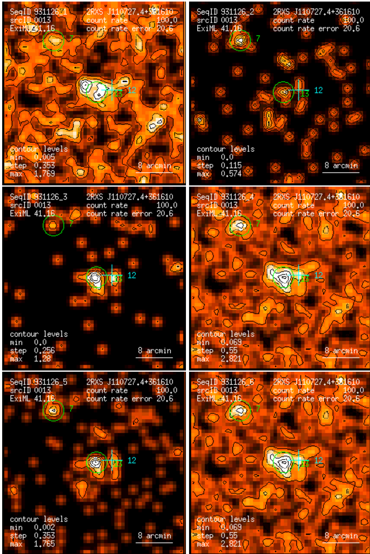
Figure 13: RASS 931126: detection 0013: band rate images, Gaussian filter: (1) PSPC channels 11 – 41, (2) 52 – 90, (3) 91 – 201, (4) 11 – 235, (5) 52 – 201, (6) 11 – 201. Broad band rates in counts/ks. Band rate contour levels in counts/ks/arcmin 2 .
