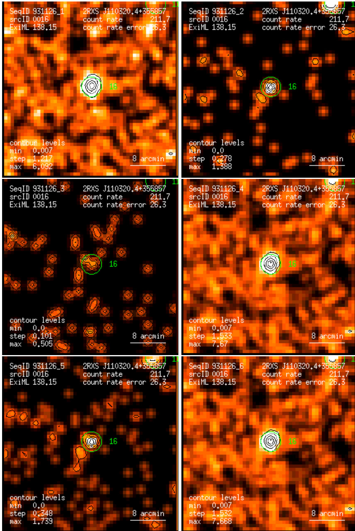
Figure 16: RASS 931126: detection 0016: band rate images, Gaussian filter: (1) PSPC channels 11 – 41, (2) 52 – 90, (3) 91 – 201, (4) 11 – 235, (5) 52 – 201, (6) 11 – 201. Broad band rates in counts/ks. Band rate contour levels in counts/ks/arcmin 2 .
