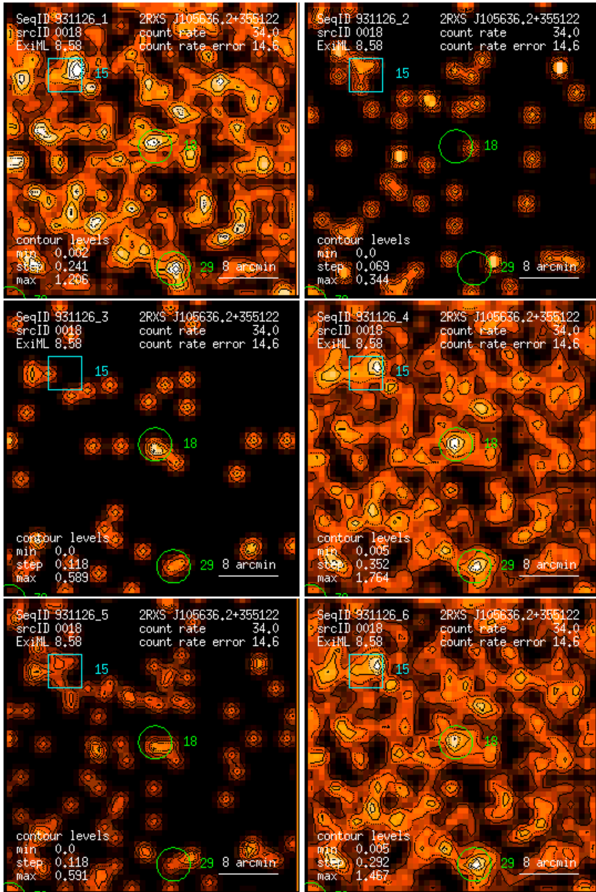
Figure 18: RASS 931126: detection 0018: band rate images, Gaussian filter: (1) PSPC channels 11 – 41, (2) 52 – 90, (3) 91 – 201, (4) 11 – 235, (5) 52 – 201, (6) 11 – 201. Broad band rates in counts/ks. Band rate contour levels in counts/ks/arcmin 2 .
