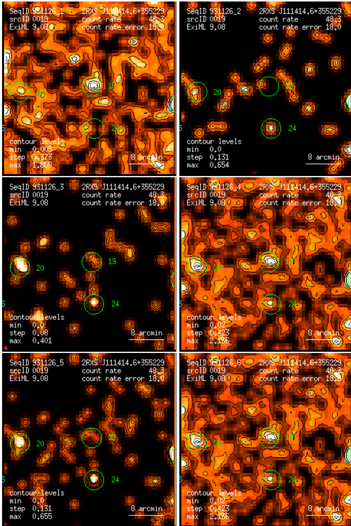
Figure 19: RASS 931126: detection 0019: band rate images, Gaussian filter: (1) PSPC channels 11 – 41, (2) 52 – 90, (3) 91 – 201, (4) 11 – 235, (5) 52 – 201, (6) 11 – 201. Broad band rates in counts/ks. Band rate contour levels in counts/ks/arcmin 2 .
