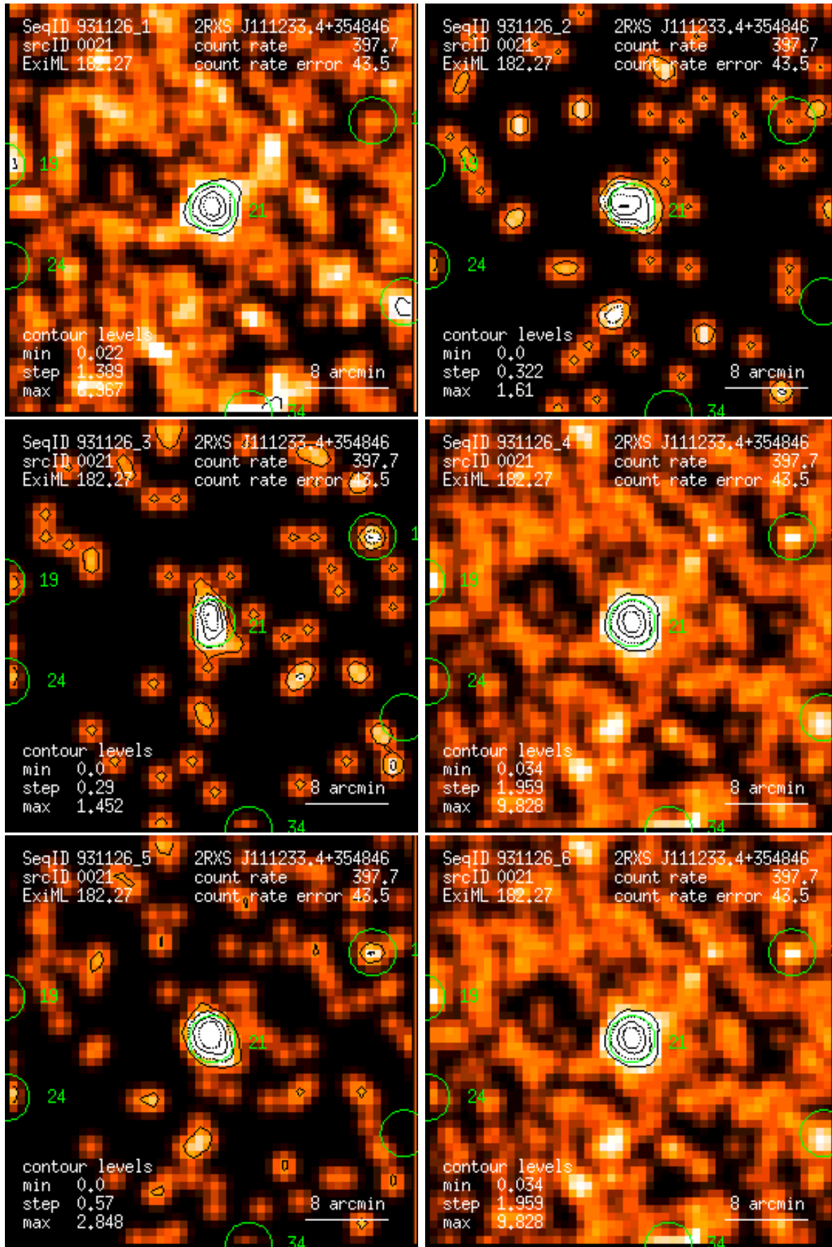
Figure 21: RASS 931126: detection 0021: band rate images, Gaussian filter: (1) PSPC channels 11 – 41, (2) 52 – 90, (3) 91 – 201, (4) 11 – 235, (5) 52 – 201, (6) 11 – 201. Broad band rates in counts/ks. Band rate contour levels in counts/ks/arcmin 2 .
