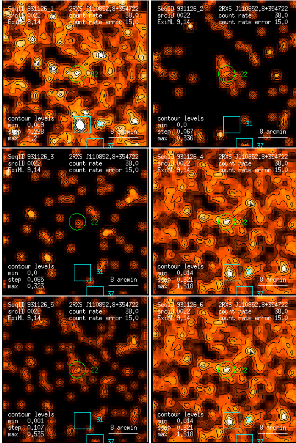
Figure 22: RASS 931126: detection 0022: band rate images, Gaussian filter: (1) PSPC channels 11 – 41, (2) 52 – 90, (3) 91 – 201, (4) 11 – 235, (5) 52 – 201, (6) 11 – 201. Broad band rates in counts/ks. Band rate contour levels in counts/ks/arcmin 2 .
