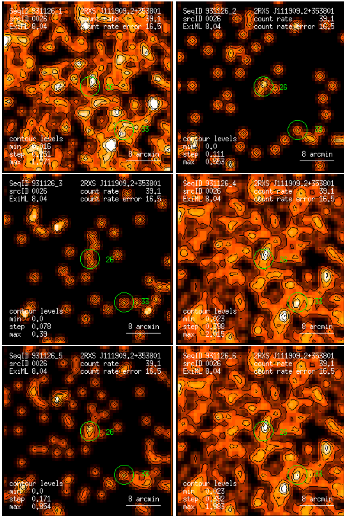
Figure 26: RASS 931126: detection 0026: band rate images, Gaussian filter: (1) PSPC channels 11 – 41, (2) 52 – 90, (3) 91 – 201, (4) 11 – 235, (5) 52 – 201, (6) 11 – 201. Broad band rates in counts/ks. Band rate contour levels in counts/ks/arcmin 2 .
