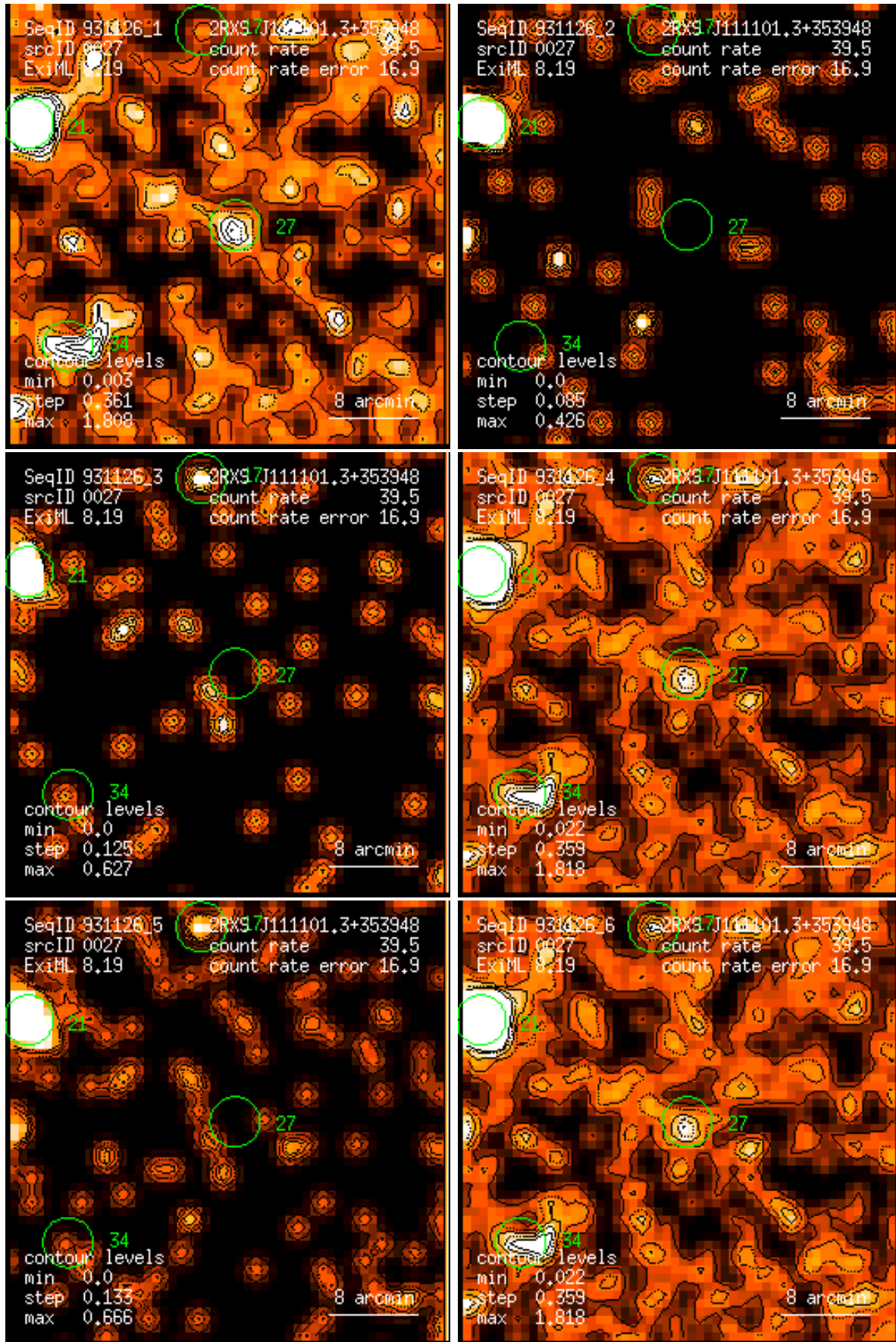
Figure 27: RASS 931126: detection 0027: band rate images, Gaussian filter: (1) PSPC channels 11 – 41, (2) 52 – 90, (3) 91 – 201, (4) 11 – 235, (5) 52 – 201, (6) 11 – 201. Broad band rates in counts/ks. Band rate contour levels in counts/ks/arcmin 2 .
