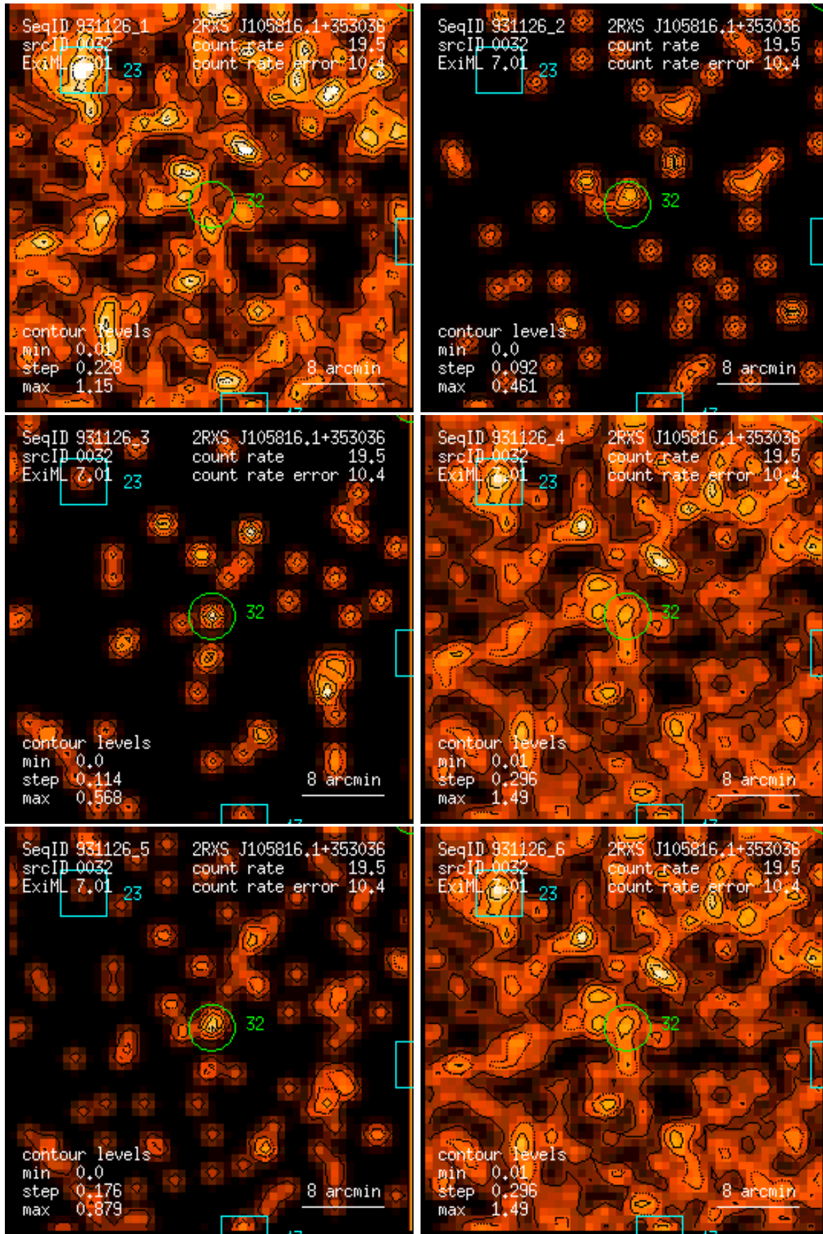
Figure 32: RASS 931126: detection 0032: band rate images, Gaussian filter: (1) PSPC channels 11 – 41, (2) 52 – 90, (3) 91 – 201, (4) 11 – 235, (5) 52 – 201, (6) 11 – 201. Broad band rates in counts/ks. Band rate contour levels in counts/ks/arcmin 2 .
