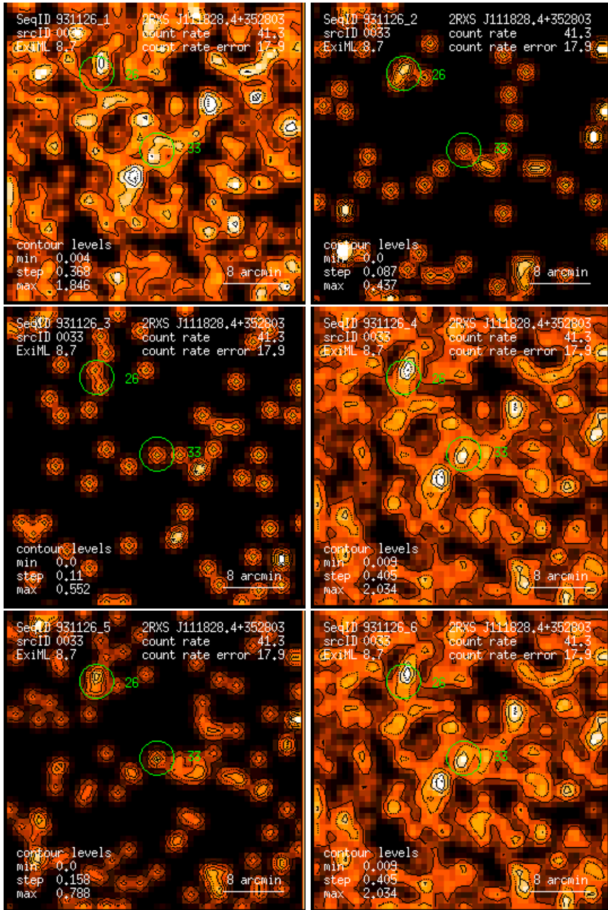
Figure 33: RASS 931126: detection 0033: band rate images, Gaussian filter: (1) PSPC channels 11 – 41, (2) 52 – 90, (3) 91 – 201, (4) 11 – 235, (5) 52 – 201, (6) 11 – 201. Broad band rates in counts/ks. Band rate contour levels in counts/ks/arcmin 2 .
