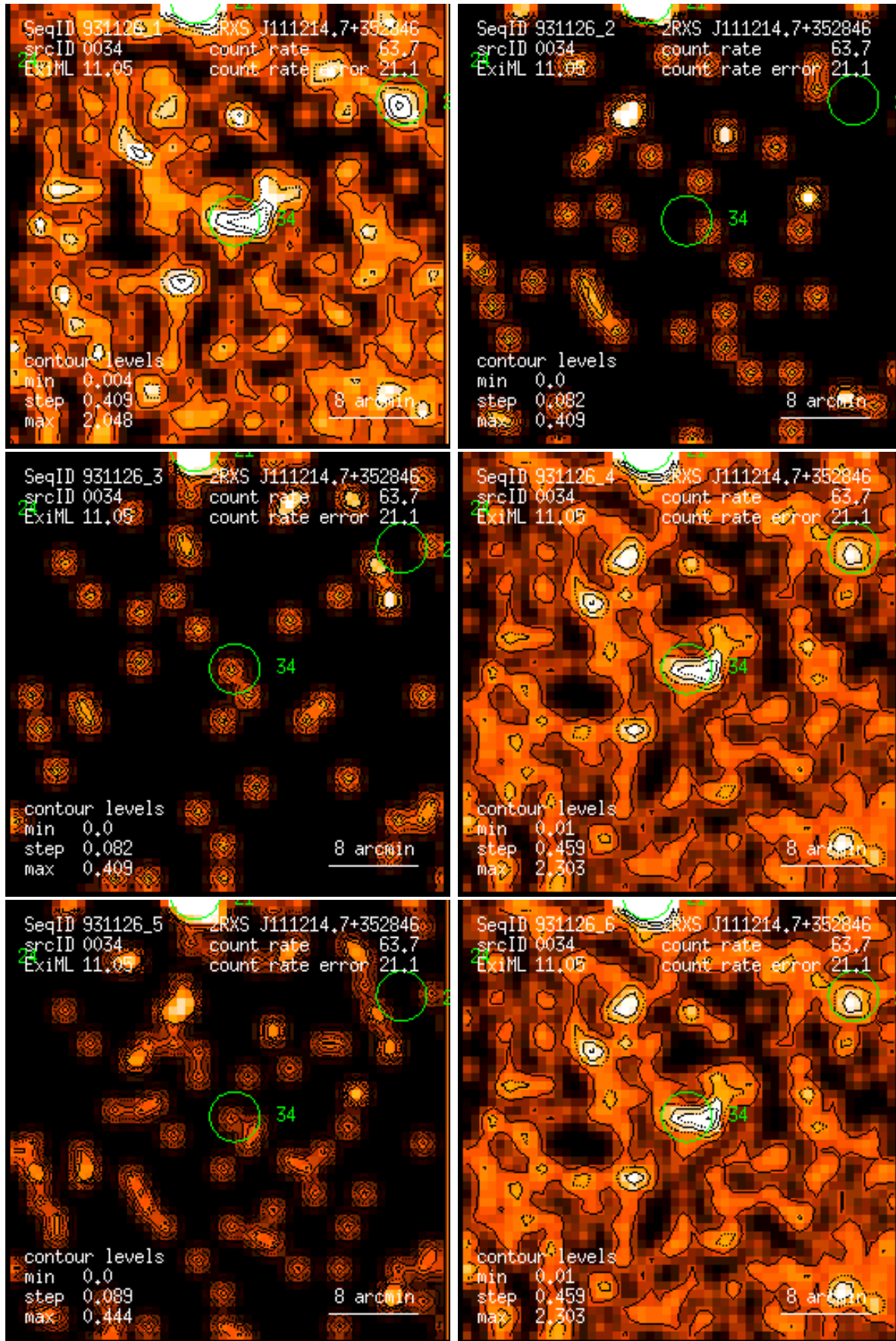
Figure 34: RASS 931126: detection 0034: band rate images, Gaussian filter: (1) PSPC channels 11 – 41, (2) 52 – 90, (3) 91 – 201, (4) 11 – 235, (5) 52 – 201, (6) 11 – 201. Broad band rates in counts/ks. Band rate contour levels in counts/ks/arcmin 2 .
