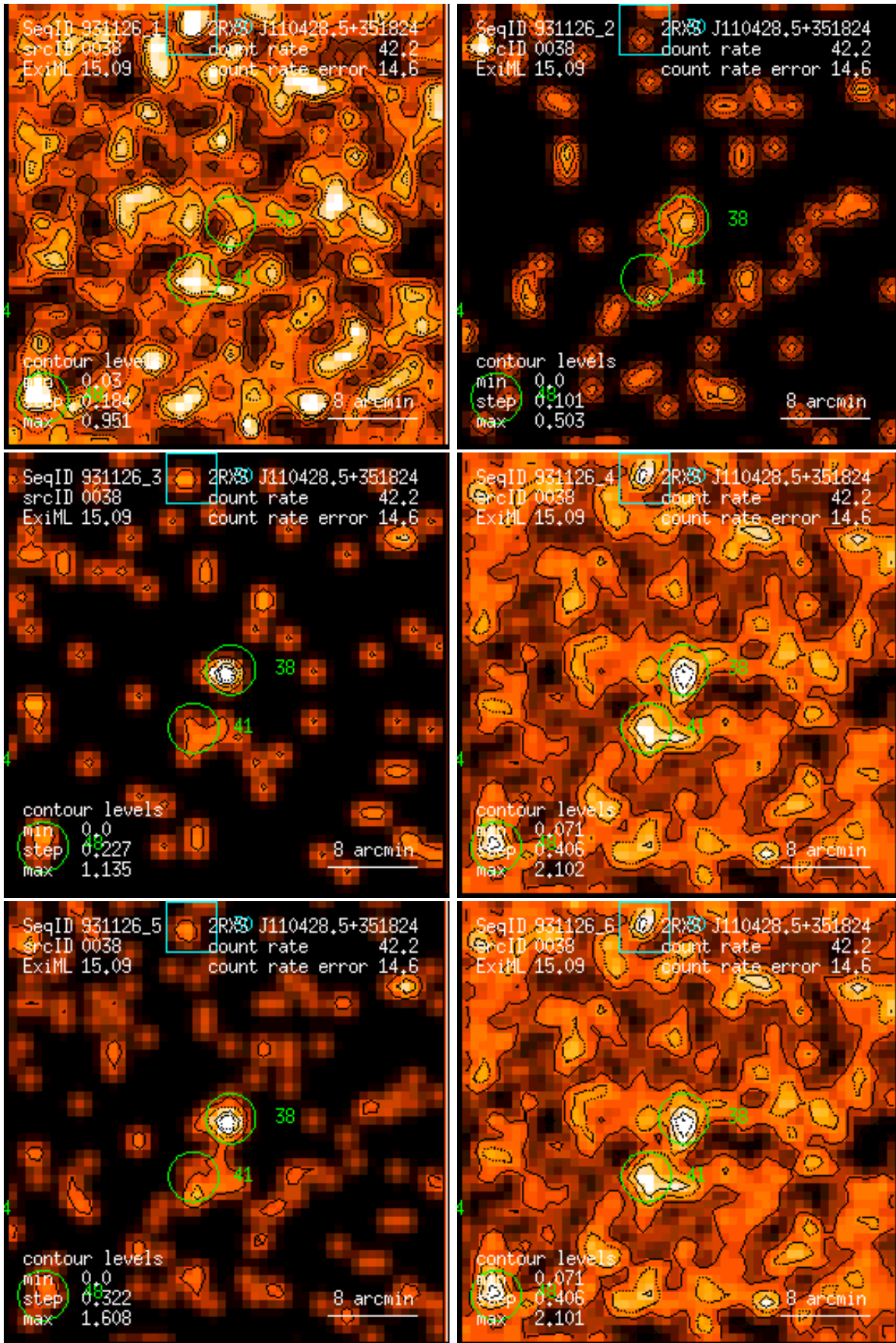
Figure 38: RASS 931126: detection 0038: band rate images, Gaussian filter: (1) PSPC channels 11 – 41, (2) 52 – 90, (3) 91 – 201, (4) 11 – 235, (5) 52 – 201, (6) 11 – 201. Broad band rates in counts/ks. Band rate contour levels in counts/ks/arcmin 2 .
