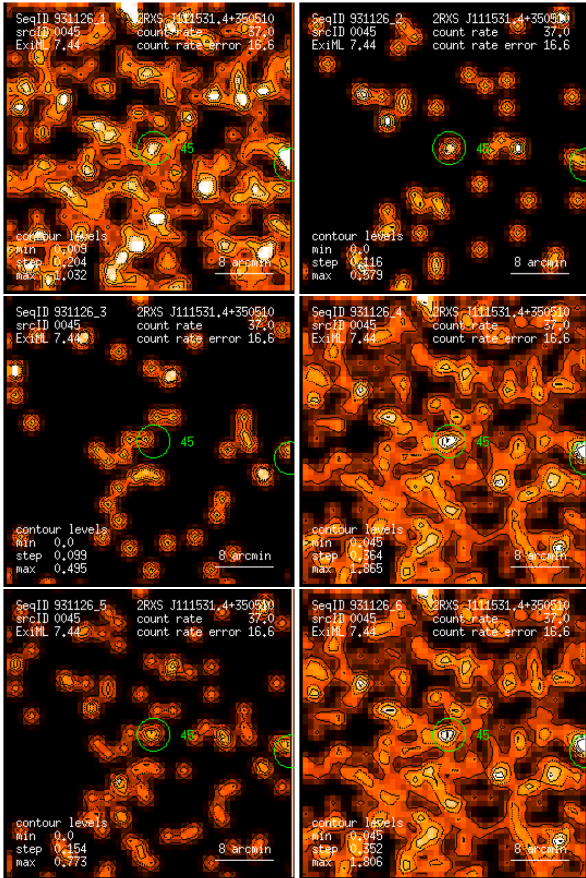
Figure 45: RASS 931126: detection 0045: band rate images, Gaussian filter: (1) PSPC channels 11 – 41, (2) 52 – 90, (3) 91 – 201, (4) 11 – 235, (5) 52 – 201, (6) 11 – 201. Broad band rates in counts/ks. Band rate contour levels in counts/ks/arcmin 2 .
