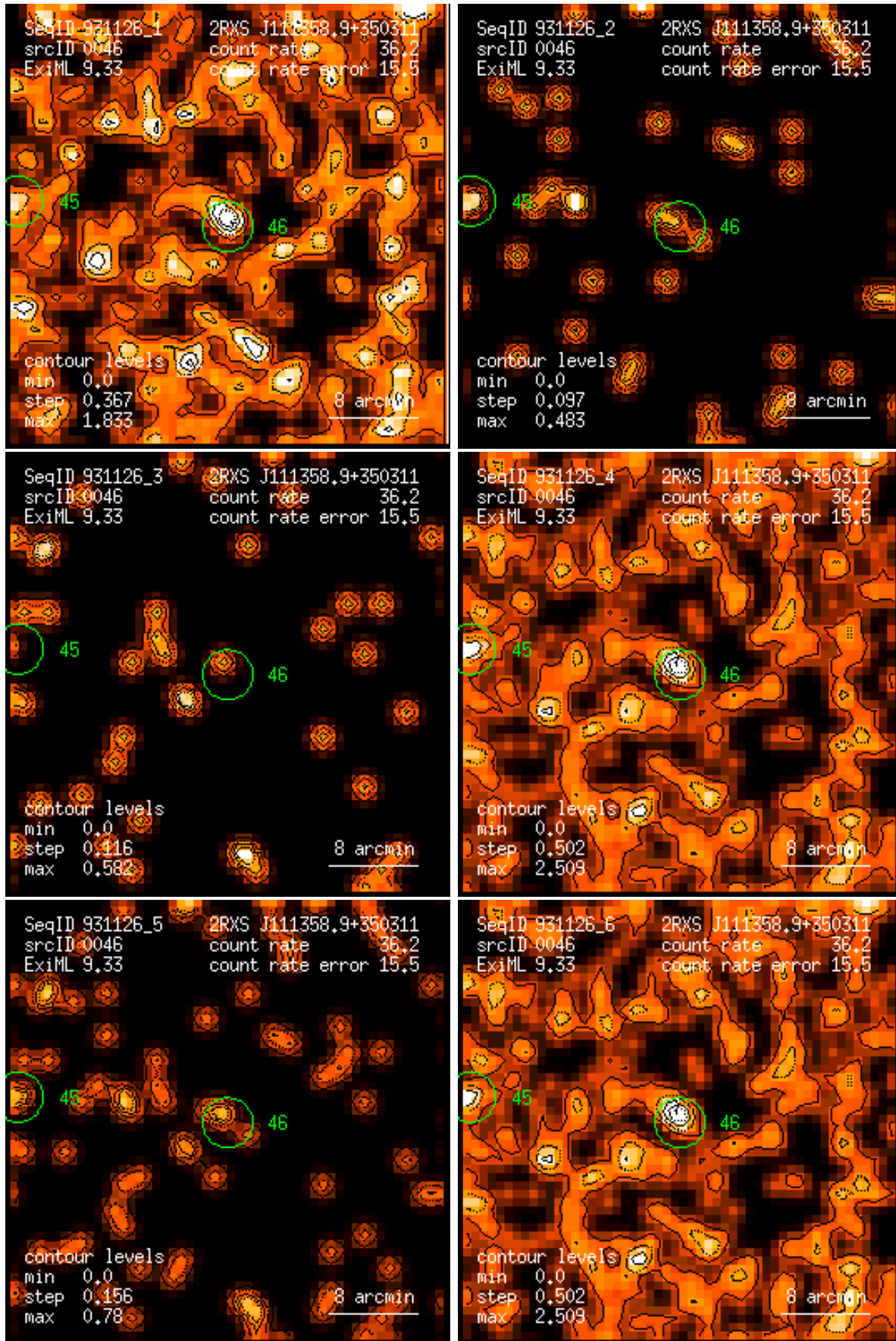
Figure 46: RASS 931126: detection 0046: band rate images, Gaussian filter: (1) PSPC channels 11 – 41, (2) 52 – 90, (3) 91 – 201, (4) 11 – 235, (5) 52 – 201, (6) 11 – 201. Broad band rates in counts/ks. Band rate contour levels in counts/ks/arcmin 2 .
