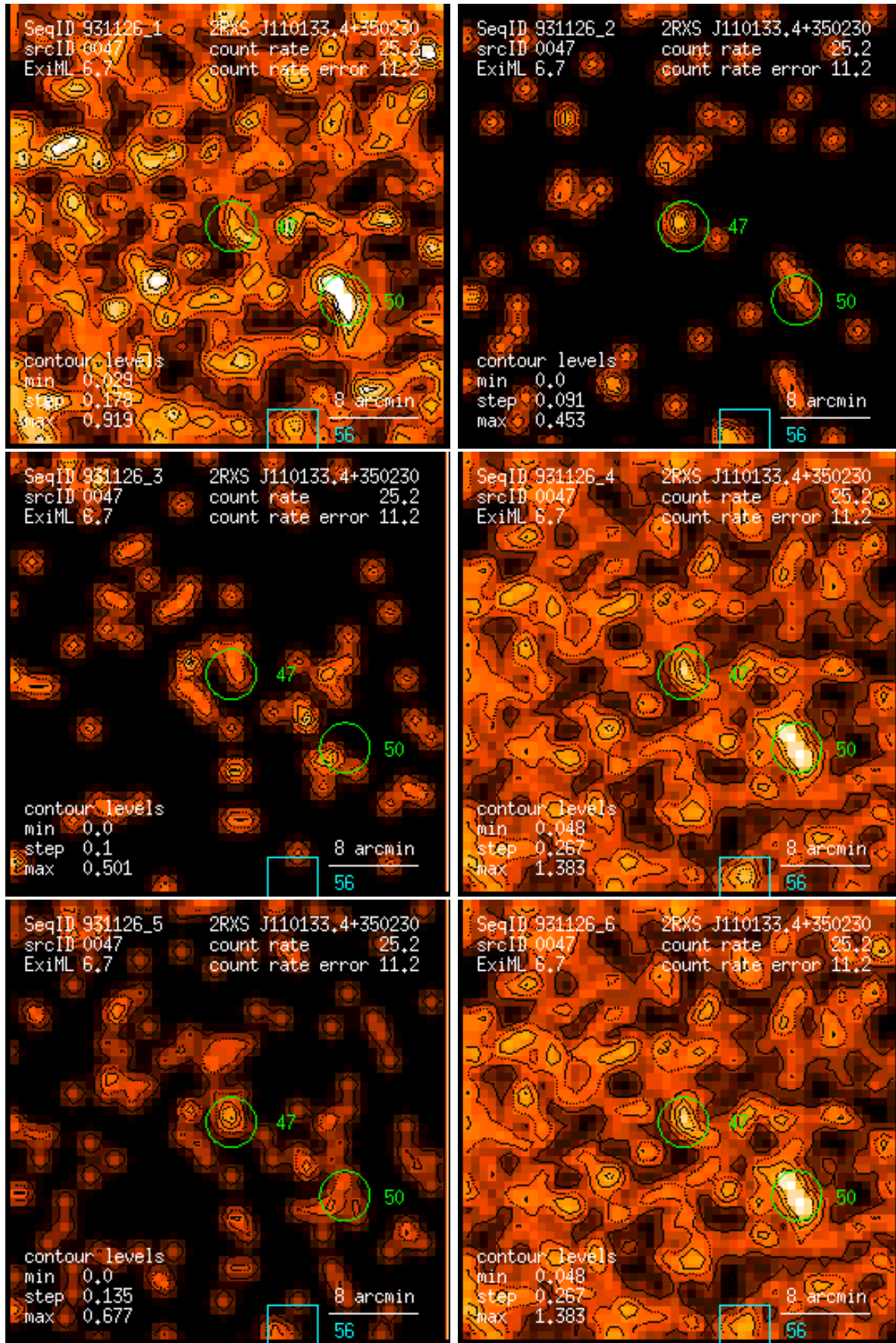
Figure 47: RASS 931126: detection 0047: band rate images, Gaussian filter: (1) PSPC channels 11 – 41, (2) 52 – 90, (3) 91 – 201, (4) 11 – 235, (5) 52 – 201, (6) 11 – 201. Broad band rates in counts/ks. Band rate contour levels in counts/ks/arcmin 2 .
