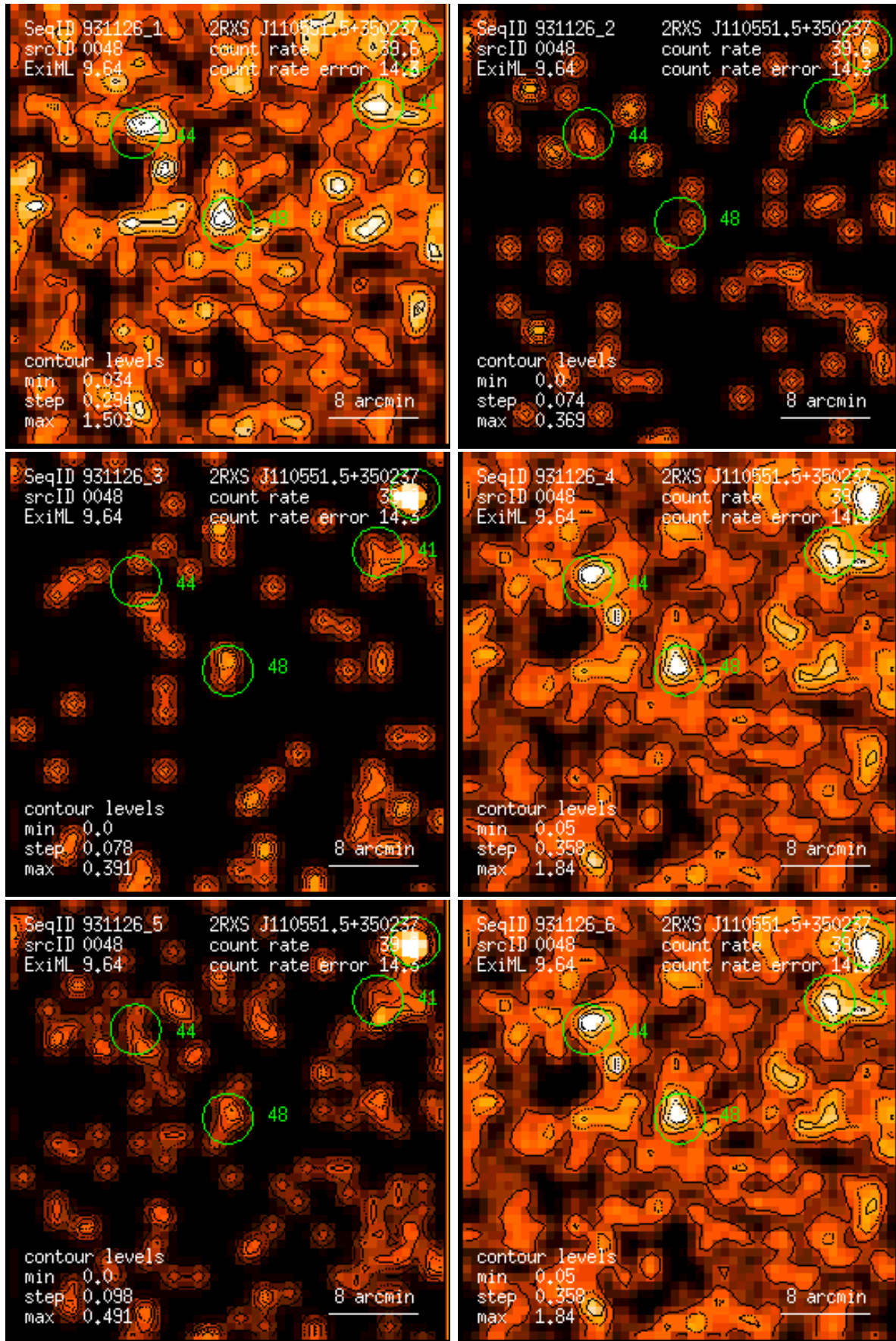
Figure 48: RASS 931126: detection 0048: band rate images, Gaussian filter: (1) PSPC channels 11 – 41, (2) 52 – 90, (3) 91 – 201, (4) 11 – 235, (5) 52 – 201, (6) 11 – 201. Broad band rates in counts/ks. Band rate contour levels in counts/ks/arcmin 2 .
