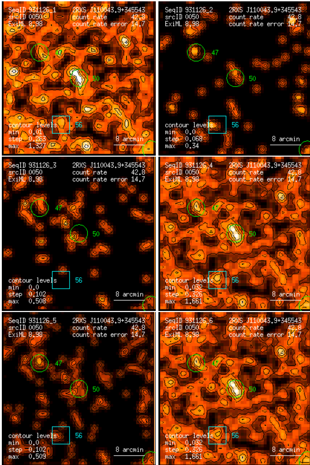
Figure 50: RASS 931126: detection 0050: band rate images, Gaussian filter: (1) PSPC channels 11 – 41, (2) 52 – 90, (3) 91 – 201, (4) 11 – 235, (5) 52 – 201, (6) 11 – 201. Broad band rates in counts/ks. Band rate contour levels in counts/ks/arcmin 2 .
