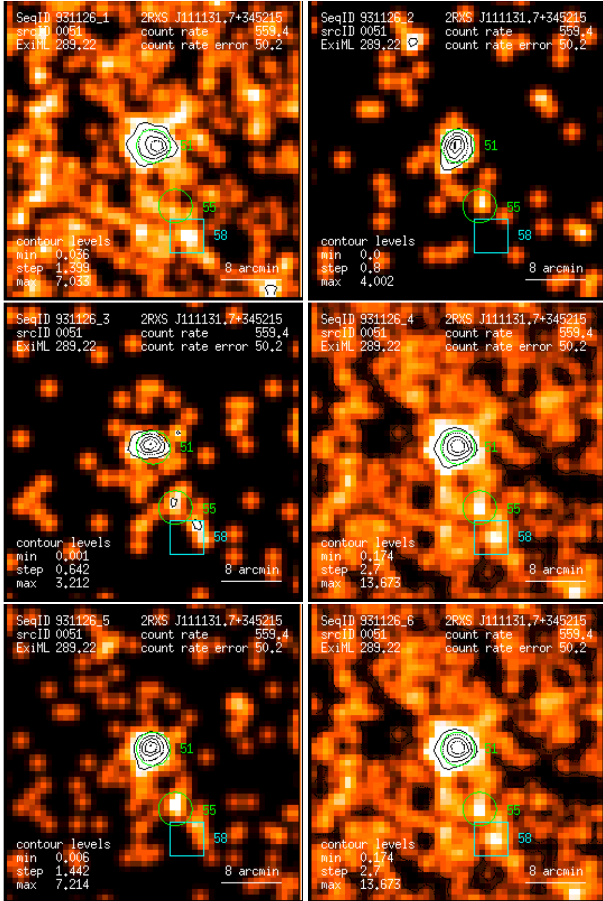
Figure 51: RASS 931126: detection 0051: band rate images, Gaussian filter: (1) PSPC channels 11 – 41, (2) 52 – 90, (3) 91 – 201, (4) 11 – 235, (5) 52 – 201, (6) 11 – 201. Broad band rates in counts/ks. Band rate contour levels in counts/ks/arcmin 2 .
