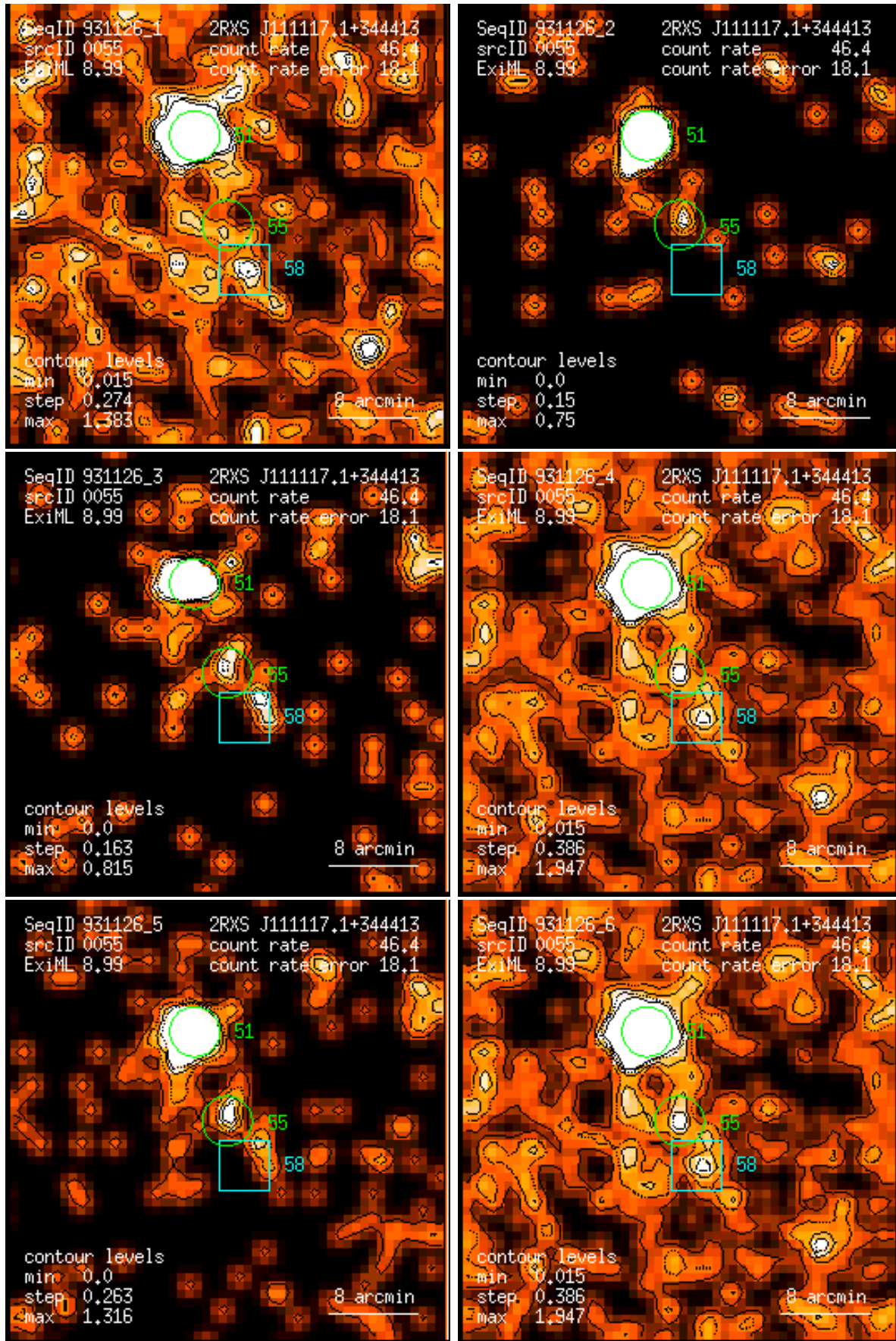
Figure 55: RASS 931126: detection 0055: band rate images, Gaussian filter: (1) PSPC channels 11 – 41, (2) 52 – 90, (3) 91 – 201, (4) 11 – 235, (5) 52 – 201, (6) 11 – 201. Broad band rates in counts/ks. Band rate contour levels in counts/ks/arcmin 2 .
