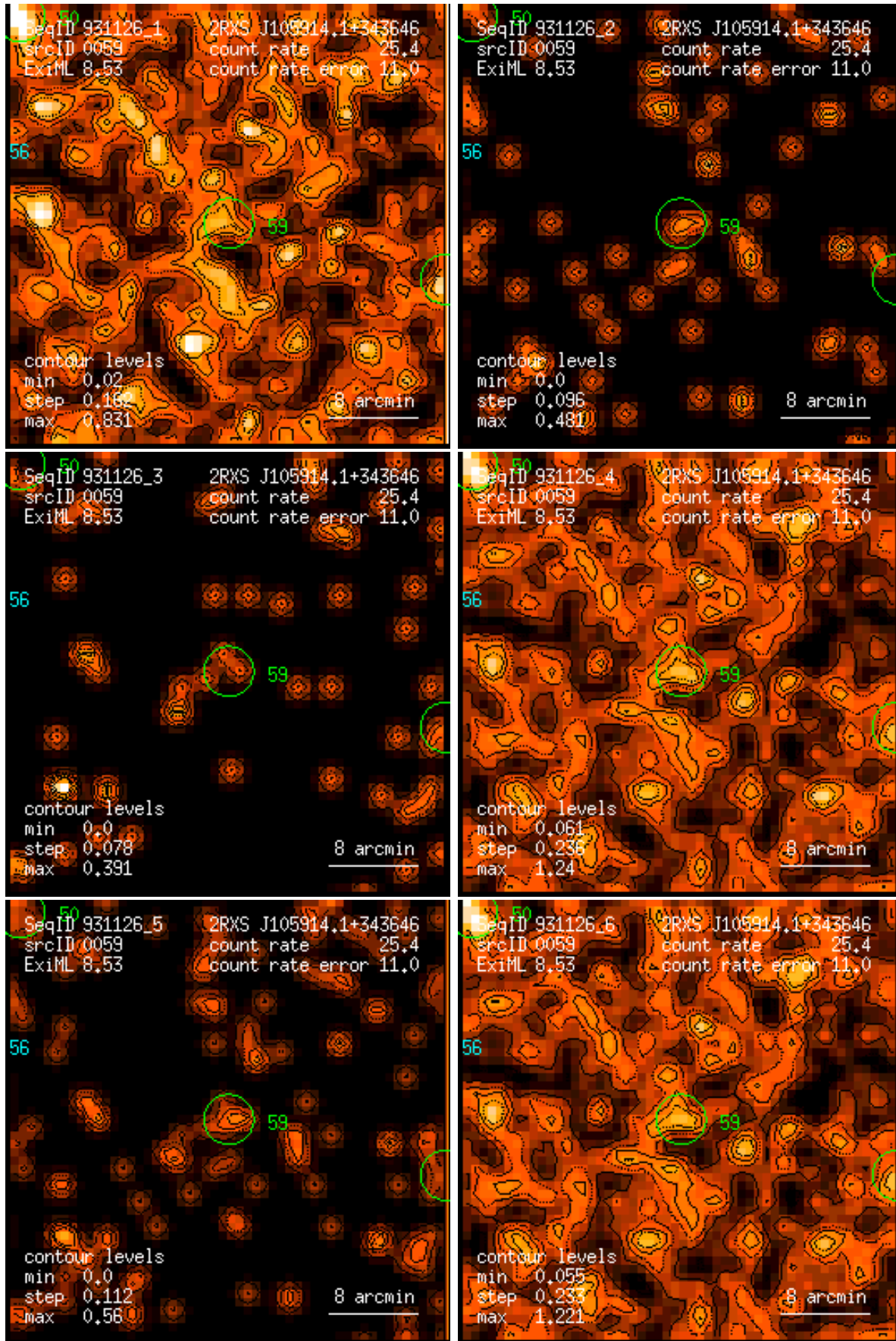
Figure 59: RASS 931126: detection 0059: band rate images, Gaussian filter: (1) PSPC channels 11 – 41, (2) 52 – 90, (3) 91 – 201, (4) 11 – 235, (5) 52 – 201, (6) 11 – 201. Broad band rates in counts/ks. Band rate contour levels in counts/ks/arcmin 2 .
