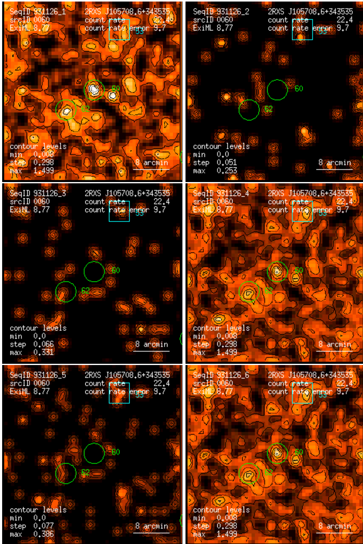
Figure 60: RASS 931126: detection 0060: band rate images, Gaussian filter: (1) PSPC channels 11 – 41, (2) 52 – 90, (3) 91 – 201, (4) 11 – 235, (5) 52 – 201, (6) 11 – 201. Broad band rates in counts/ks. Band rate contour levels in counts/ks/arcmin 2 .
