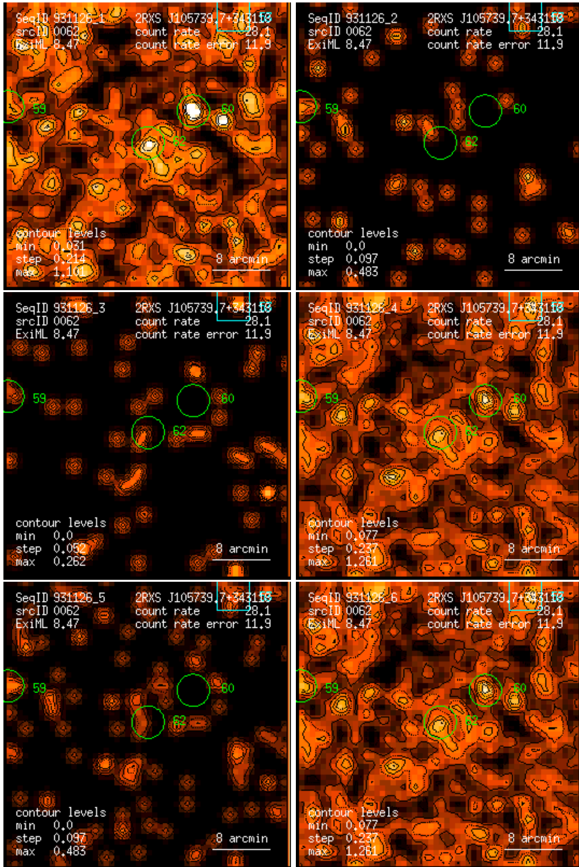
Figure 62: RASS 931126: detection 0062: band rate images, Gaussian filter: (1) PSPC channels 11 – 41, (2) 52 – 90, (3) 91 – 201, (4) 11 – 235, (5) 52 – 201, (6) 11 – 201. Broad band rates in counts/ks. Band rate contour levels in counts/ks/arcmin 2 .
