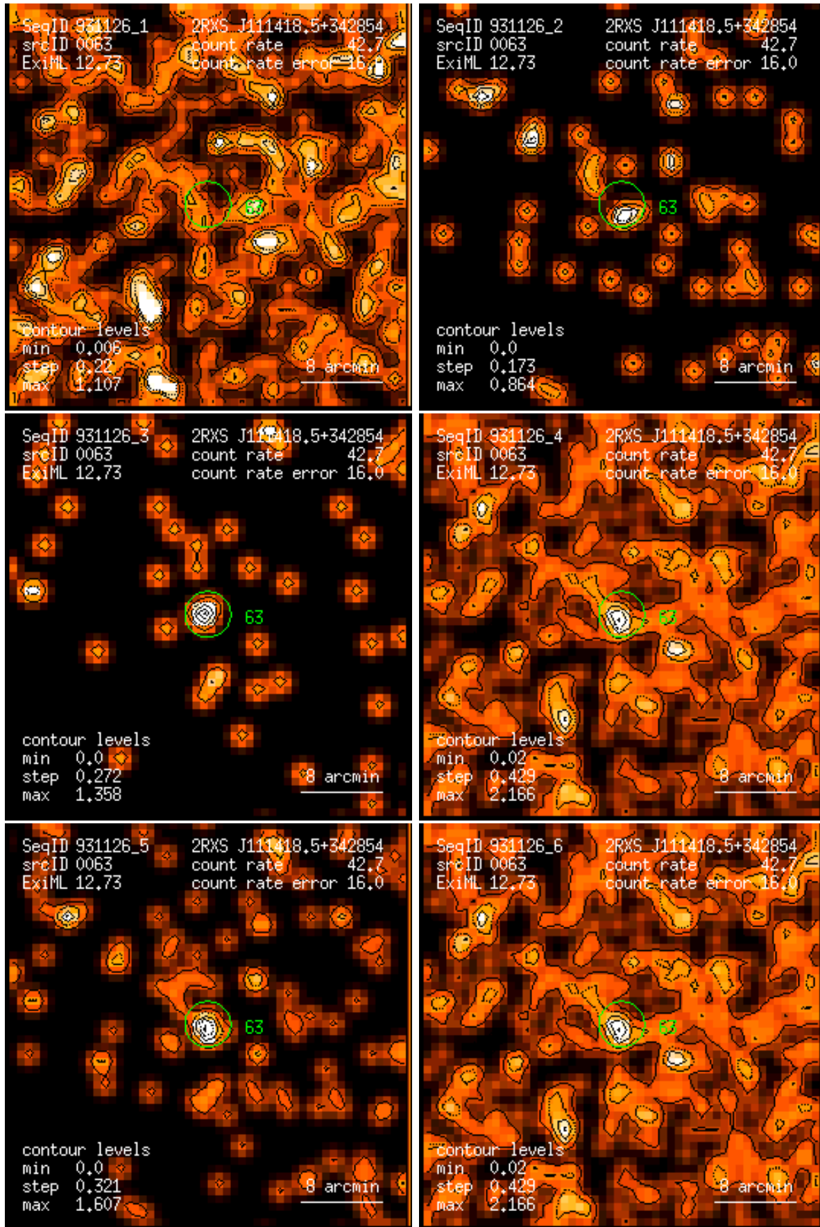
Figure 63: RASS 931126: detection 0063: band rate images, Gaussian filter: (1) PSPC channels 11 – 41, (2) 52 – 90, (3) 91 – 201, (4) 11 – 235, (5) 52 – 201, (6) 11 – 201. Broad band rates in counts/ks. Band rate contour levels in counts/ks/arcmin 2 .
