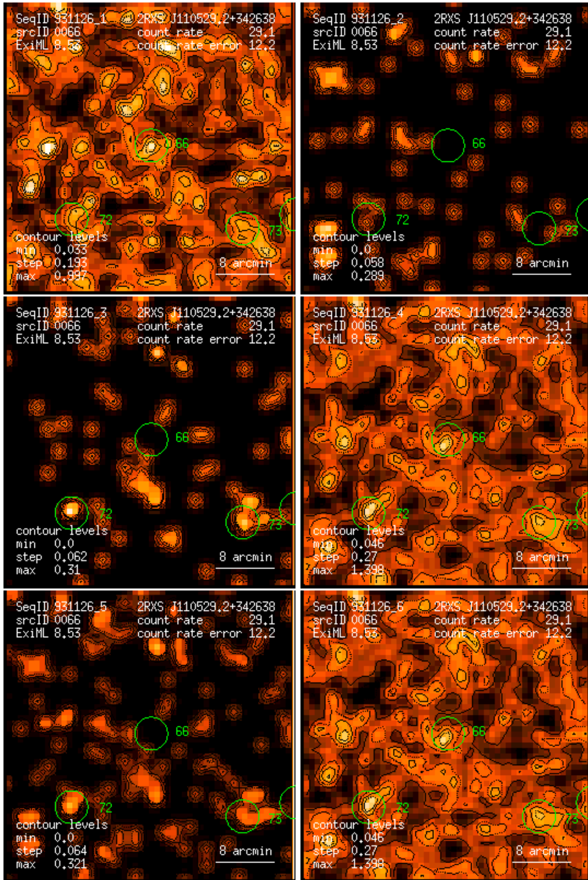
Figure 66: RASS 931126: detection 0066: band rate images, Gaussian filter: (1) PSPC channels 11 – 41, (2) 52 – 90, (3) 91 – 201, (4) 11 – 235, (5) 52 – 201, (6) 11 – 201. Broad band rates in counts/ks. Band rate contour levels in counts/ks/arcmin 2 .
