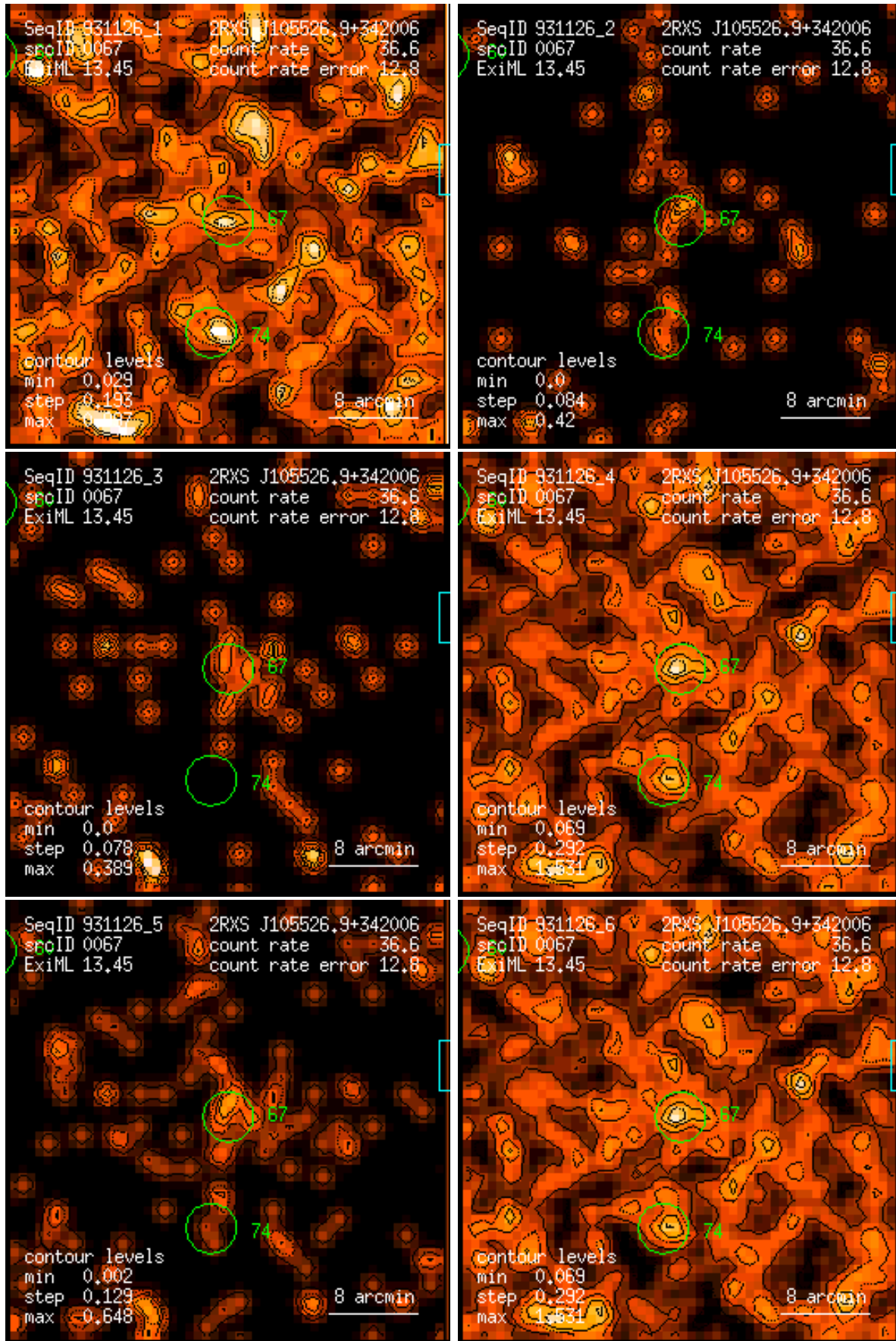
Figure 67: RASS 931126: detection 0067: band rate images, Gaussian filter: (1) PSPC channels 11 – 41, (2) 52 – 90, (3) 91 – 201, (4) 11 – 235, (5) 52 – 201, (6) 11 – 201. Broad band rates in counts/ks. Band rate contour levels in counts/ks/arcmin 2 .
