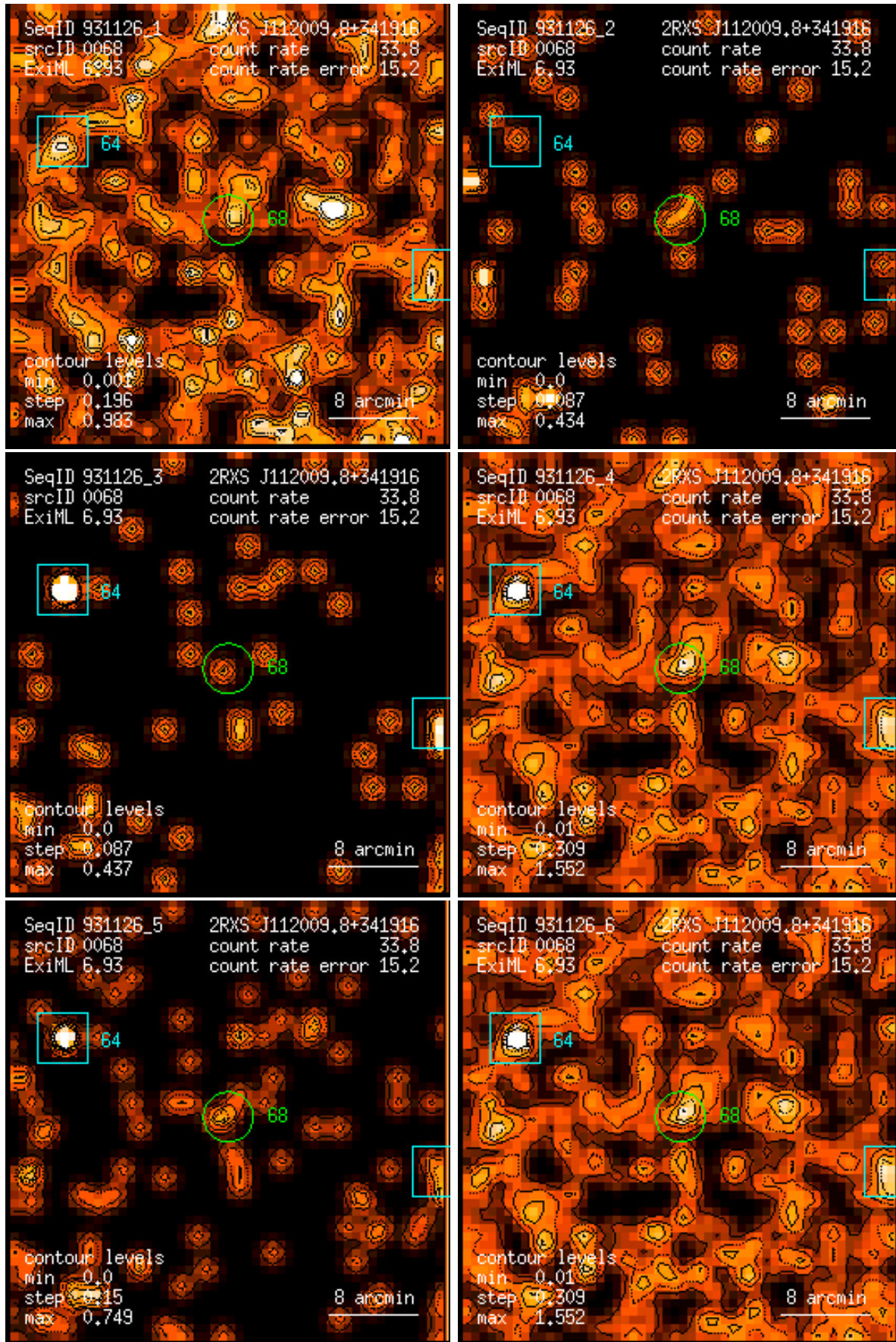
Figure 68: RASS 931126: detection 0068: band rate images, Gaussian filter: (1) PSPC channels 11 – 41, (2) 52 – 90, (3) 91 – 201, (4) 11 – 235, (5) 52 – 201, (6) 11 – 201. Broad band rates in counts/ks. Band rate contour levels in counts/ks/arcmin 2 .
