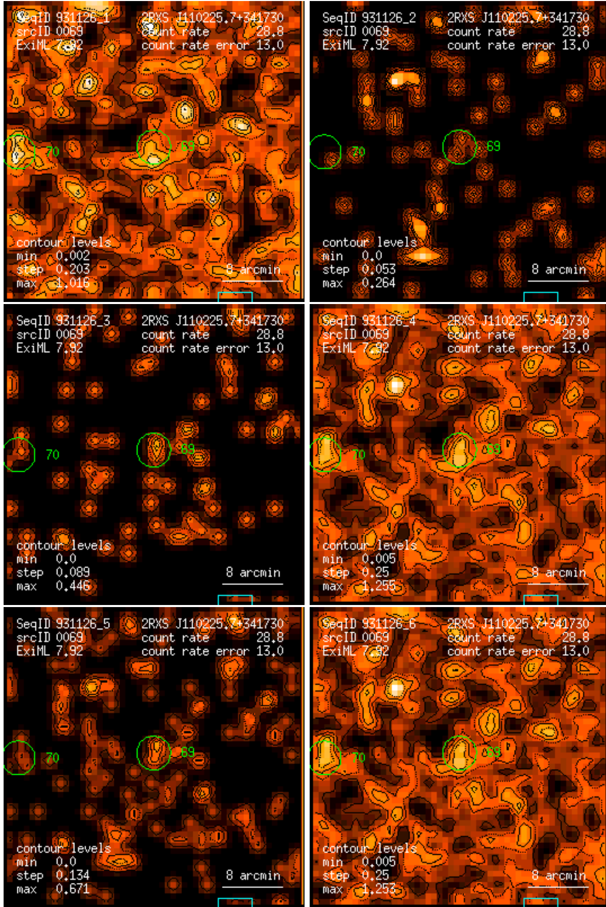
Figure 69: RASS 931126: detection 0069: band rate images, Gaussian filter: (1) PSPC channels 11 – 41, (2) 52 – 90, (3) 91 – 201, (4) 11 – 235, (5) 52 – 201, (6) 11 – 201. Broad band rates in counts/ks. Band rate contour levels in counts/ks/arcmin 2 .
