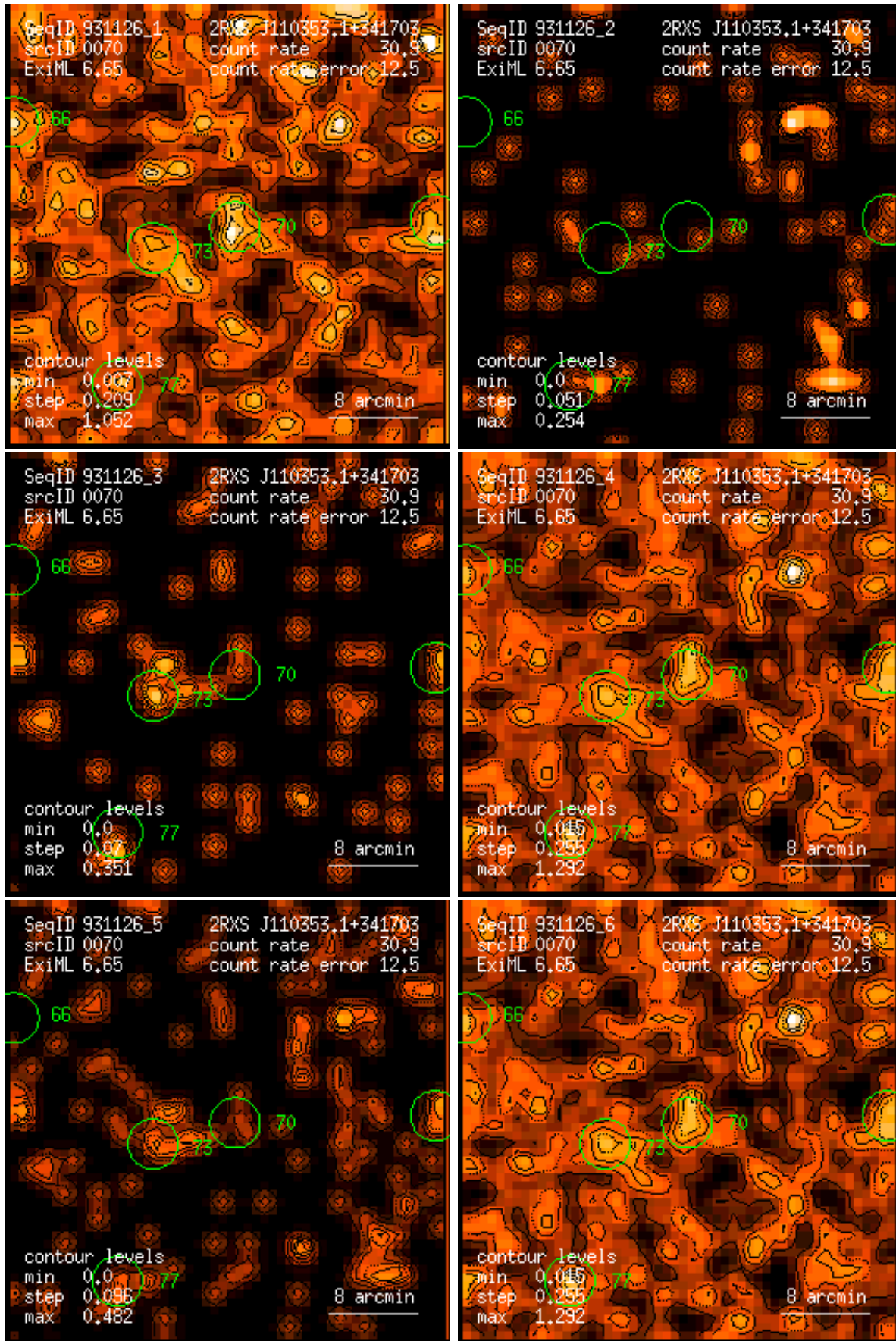
Figure 70: RASS 931126: detection 0070: band rate images, Gaussian filter: (1) PSPC channels 11 – 41, (2) 52 – 90, (3) 91 – 201, (4) 11 – 235, (5) 52 – 201, (6) 11 – 201. Broad band rates in counts/ks. Band rate contour levels in counts/ks/arcmin 2 .
