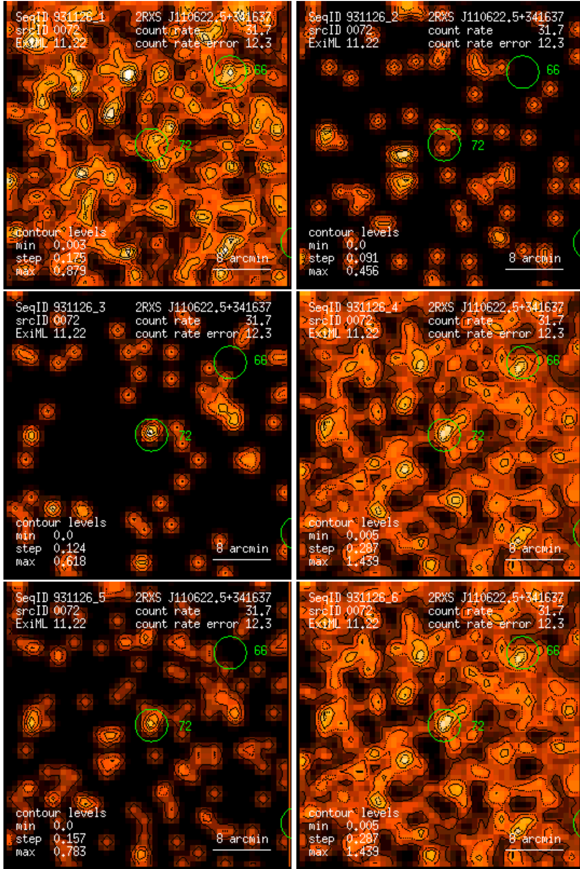
Figure 72: RASS 931126: detection 0072: band rate images, Gaussian filter: (1) PSPC channels 11 – 41, (2) 52 – 90, (3) 91 – 201, (4) 11 – 235, (5) 52 – 201, (6) 11 – 201. Broad band rates in counts/ks. Band rate contour levels in counts/ks/arcmin 2 .
