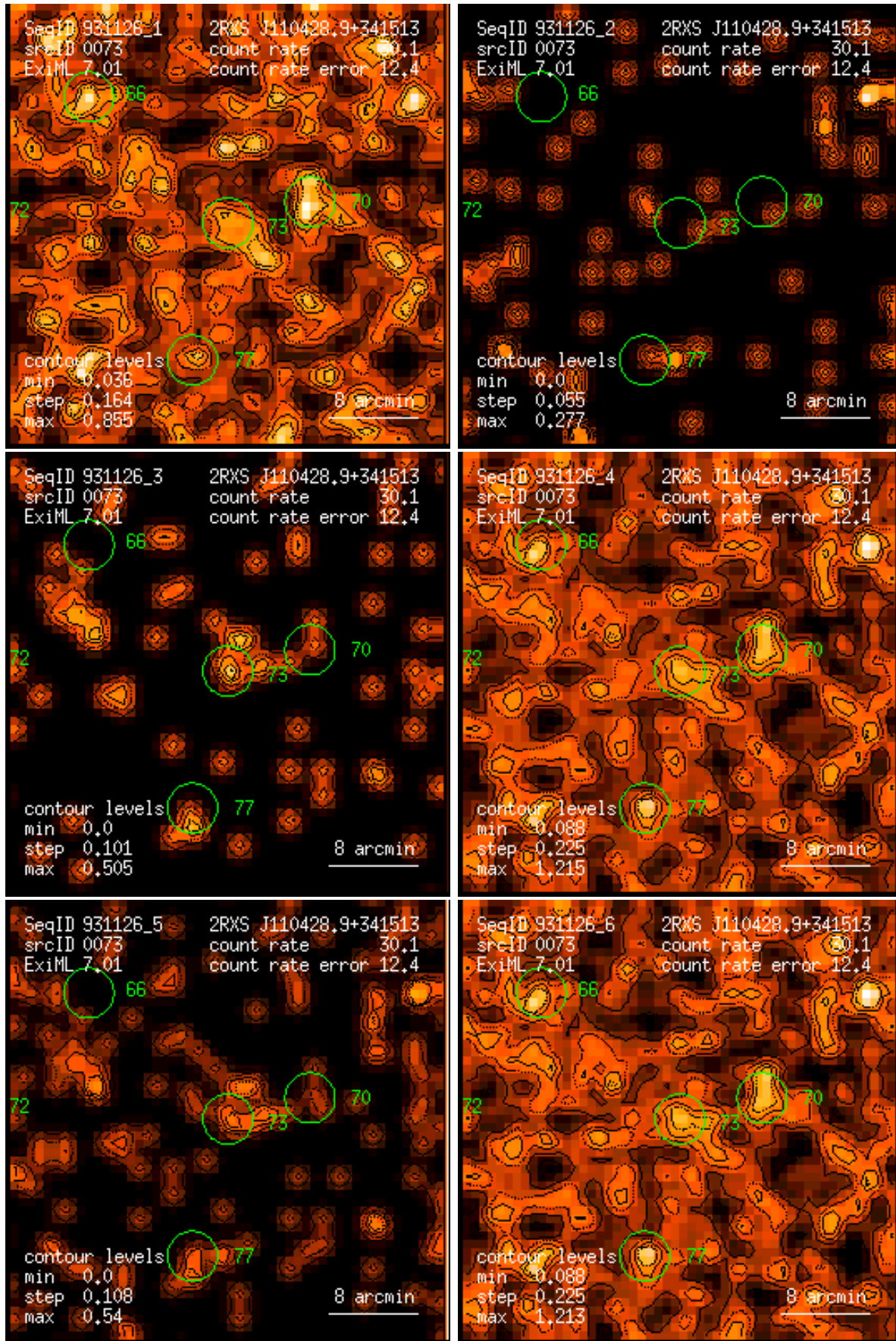
Figure 73: RASS 931126: detection 0073: band rate images, Gaussian filter: (1) PSPC channels 11 – 41, (2) 52 – 90, (3) 91 – 201, (4) 11 – 235, (5) 52 – 201, (6) 11 – 201. Broad band rates in counts/ks. Band rate contour levels in counts/ks/arcmin 2 .
