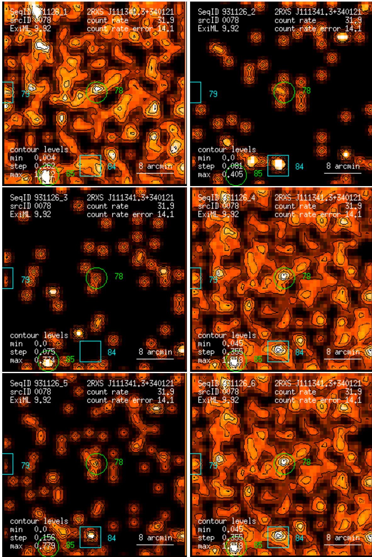
Figure 78: RASS 931126: detection 0078: band rate images, Gaussian filter: (1) PSPC channels 11 – 41, (2) 52 – 90, (3) 91 – 201, (4) 11 – 235, (5) 52 – 201, (6) 11 – 201. Broad band rates in counts/ks. Band rate contour levels in counts/ks/arcmin 2 .
