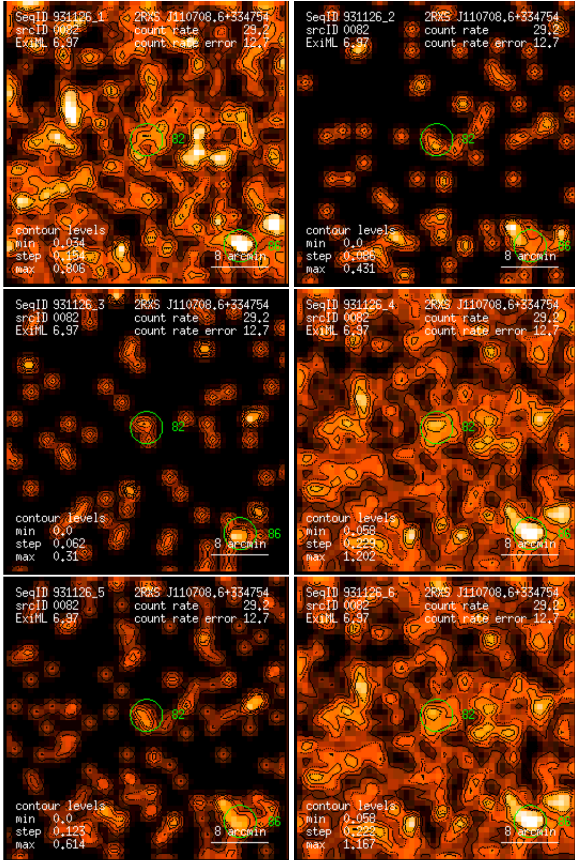
Figure 82: RASS 931126: detection 0082: band rate images, Gaussian filter: (1) PSPC channels 11 – 41, (2) 52 – 90, (3) 91 – 201, (4) 11 – 235, (5) 52 – 201, (6) 11 – 201. Broad band rates in counts/ks. Band rate contour levels in counts/ks/arcmin 2 .
