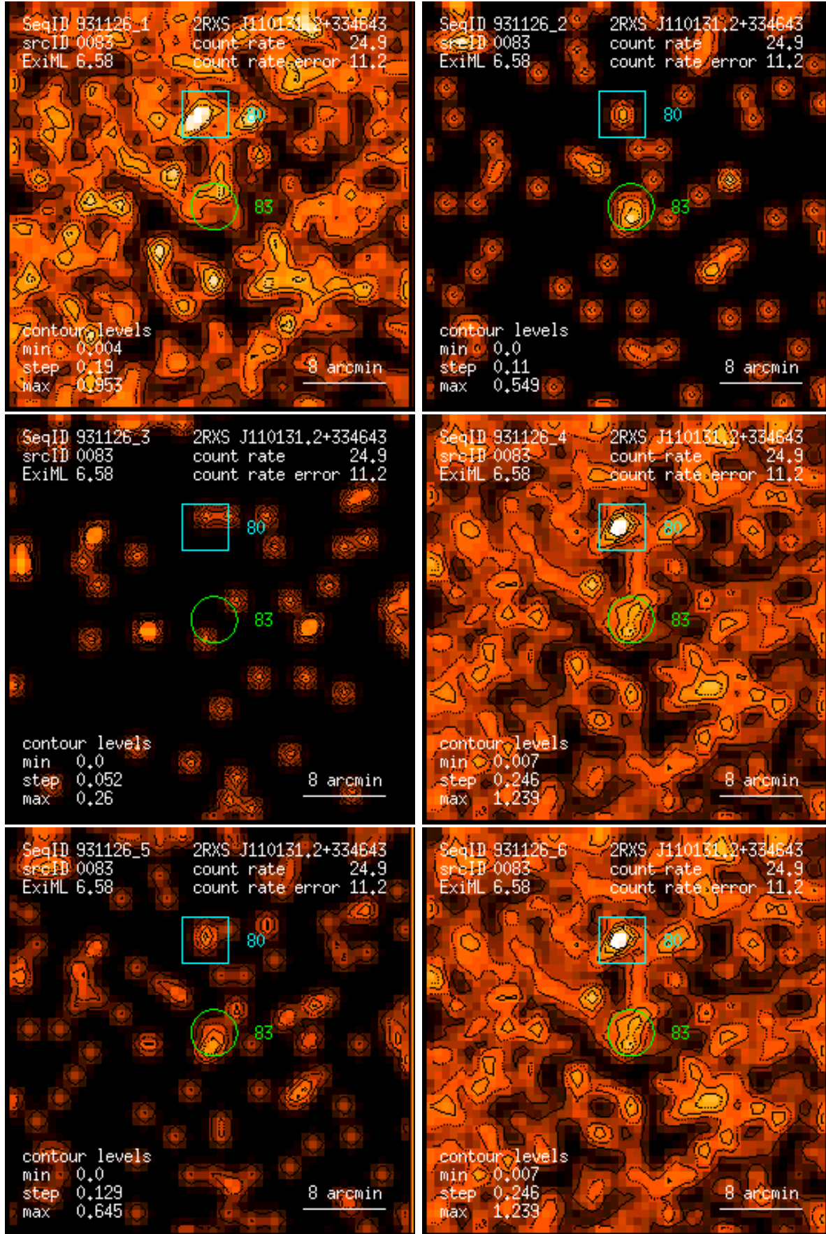
Figure 83: RASS 931126: detection 0083: band rate images, Gaussian filter: (1) PSPC channels 11 – 41, (2) 52 – 90, (3) 91 – 201, (4) 11 – 235, (5) 52 – 201, (6) 11 – 201. Broad band rates in counts/ks. Band rate contour levels in counts/ks/arcmin 2 .
