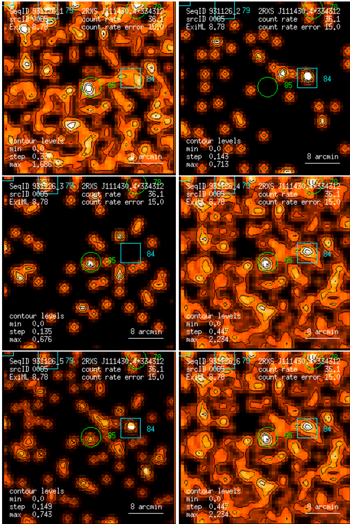
Figure 85: RASS 931126: detection 0085: band rate images, Gaussian filter: (1) PSPC channels 11 – 41, (2) 52 – 90, (3) 91 – 201, (4) 11 – 235, (5) 52 – 201, (6) 11 – 201. Broad band rates in counts/ks. Band rate contour levels in counts/ks/arcmin 2 .
