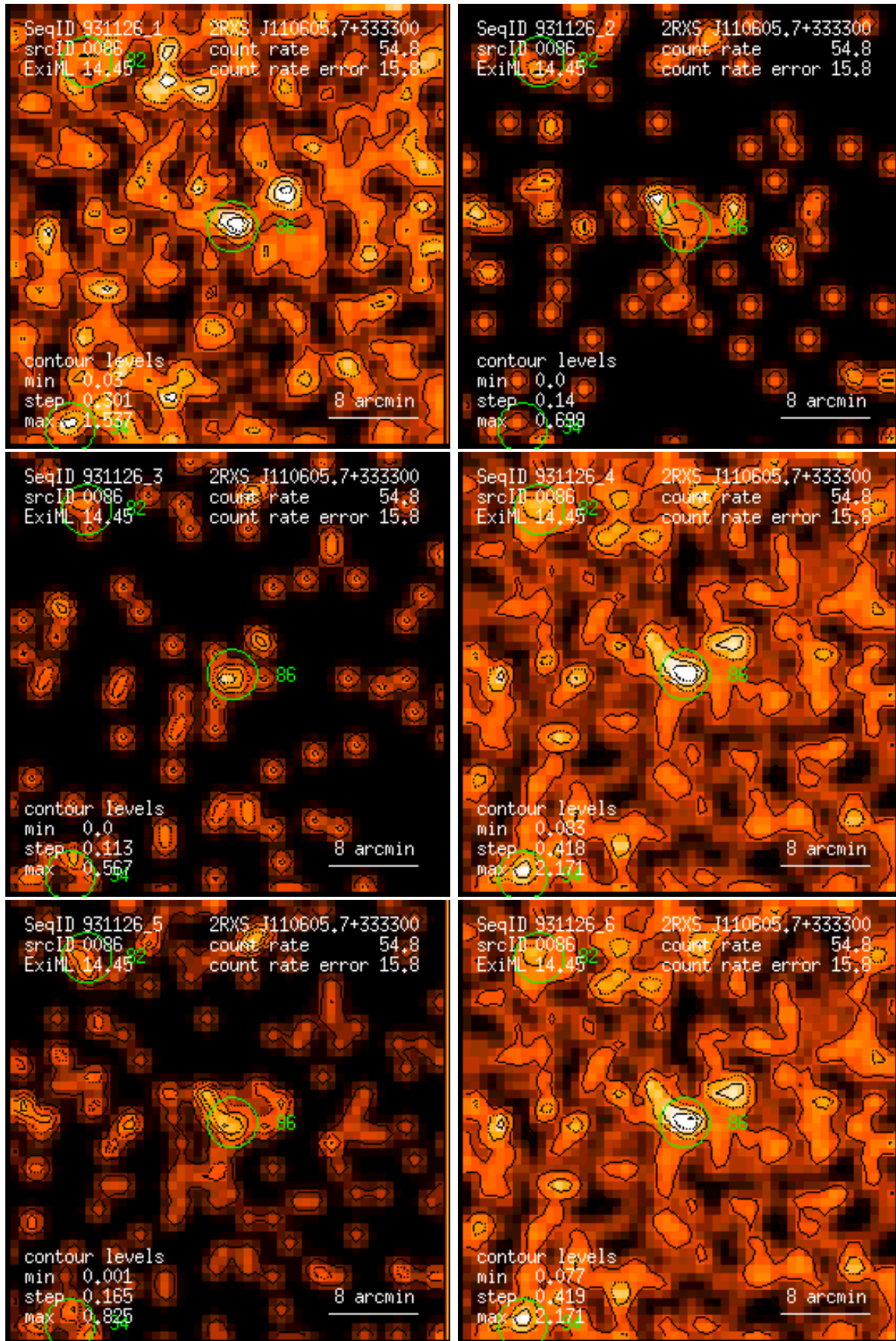
Figure 86: RASS 931126: detection 0086: band rate images, Gaussian filter: (1) PSPC channels 11 – 41, (2) 52 – 90, (3) 91 – 201, (4) 11 – 235, (5) 52 – 201, (6) 11 – 201. Broad band rates in counts/ks. Band rate contour levels in counts/ks/arcmin 2 .
