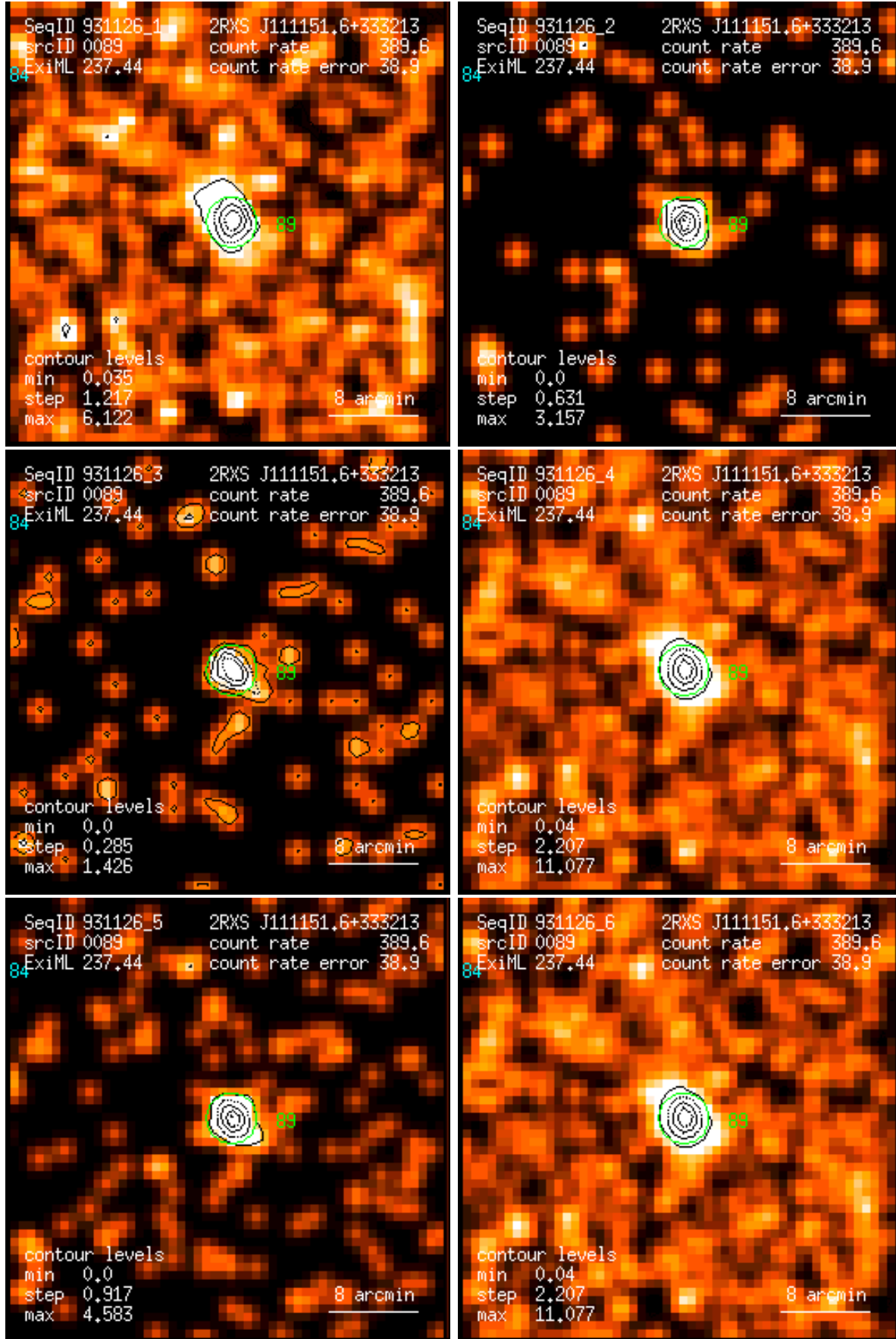
Figure 89: RASS 931126: detection 0089: band rate images, Gaussian filter: (1) PSPC channels 11 – 41, (2) 52 – 90, (3) 91 – 201, (4) 11 – 235, (5) 52 – 201, (6) 11 – 201. Broad band rates in counts/ks. Band rate contour levels in counts/ks/arcmin 2 .
