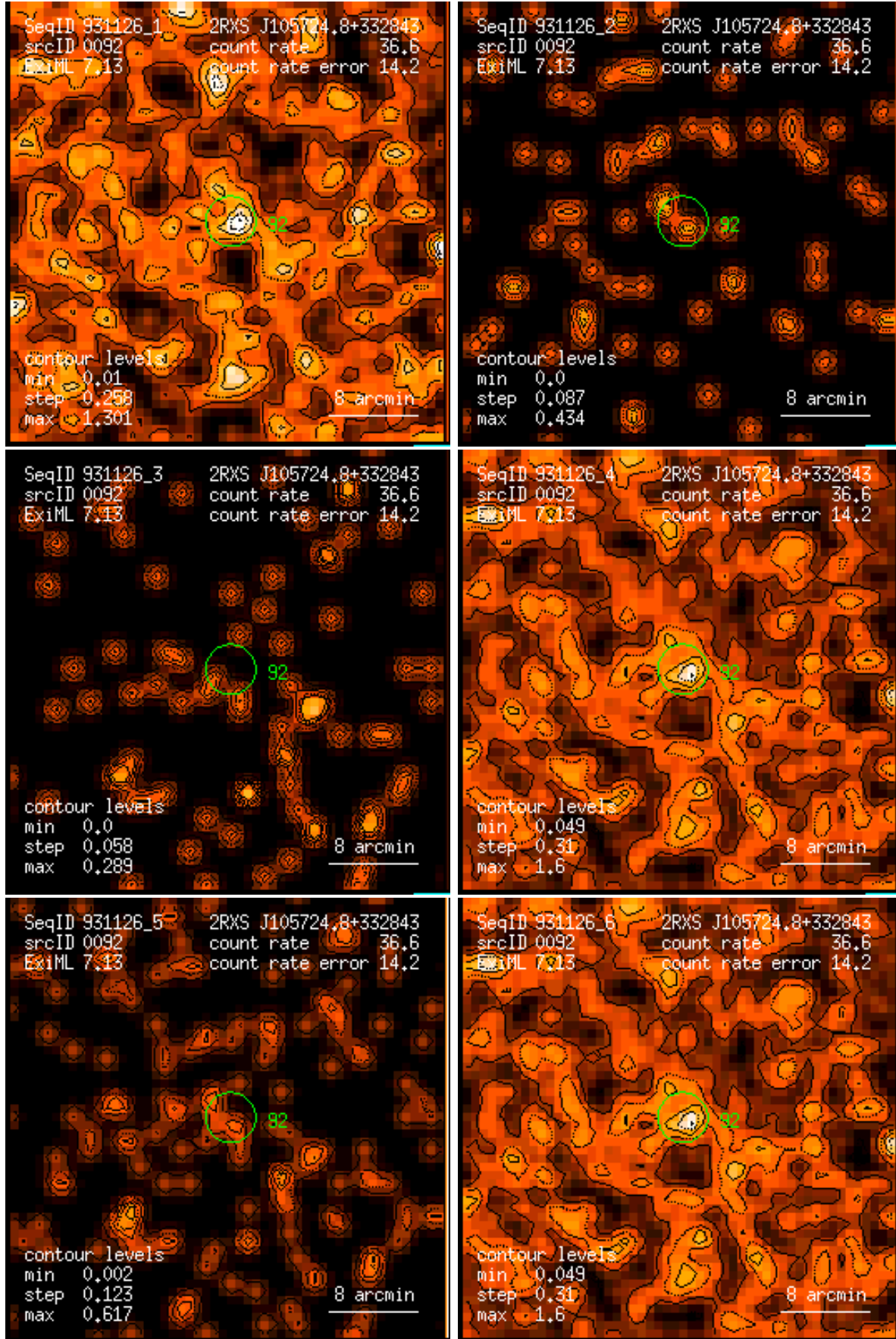
Figure 92: RASS 931126: detection 0092: band rate images, Gaussian filter: (1) PSPC channels 11 – 41, (2) 52 – 90, (3) 91 – 201, (4) 11 – 235, (5) 52 – 201, (6) 11 – 201. Broad band rates in counts/ks. Band rate contour levels in counts/ks/arcmin 2 .
