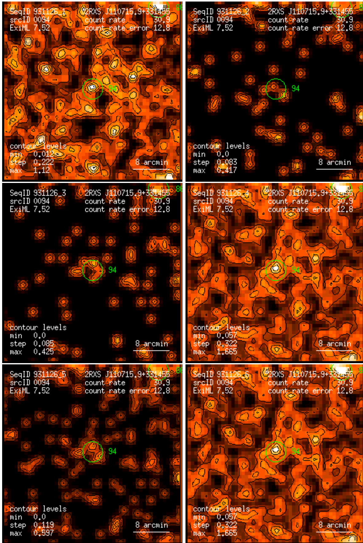
Figure 94: RASS 931126: detection 0094: band rate images, Gaussian filter: (1) PSPC channels 11 – 41, (2) 52 – 90, (3) 91 – 201, (4) 11 – 235, (5) 52 – 201, (6) 11 – 201. Broad band rates in counts/ks. Band rate contour levels in counts/ks/arcmin 2 .
