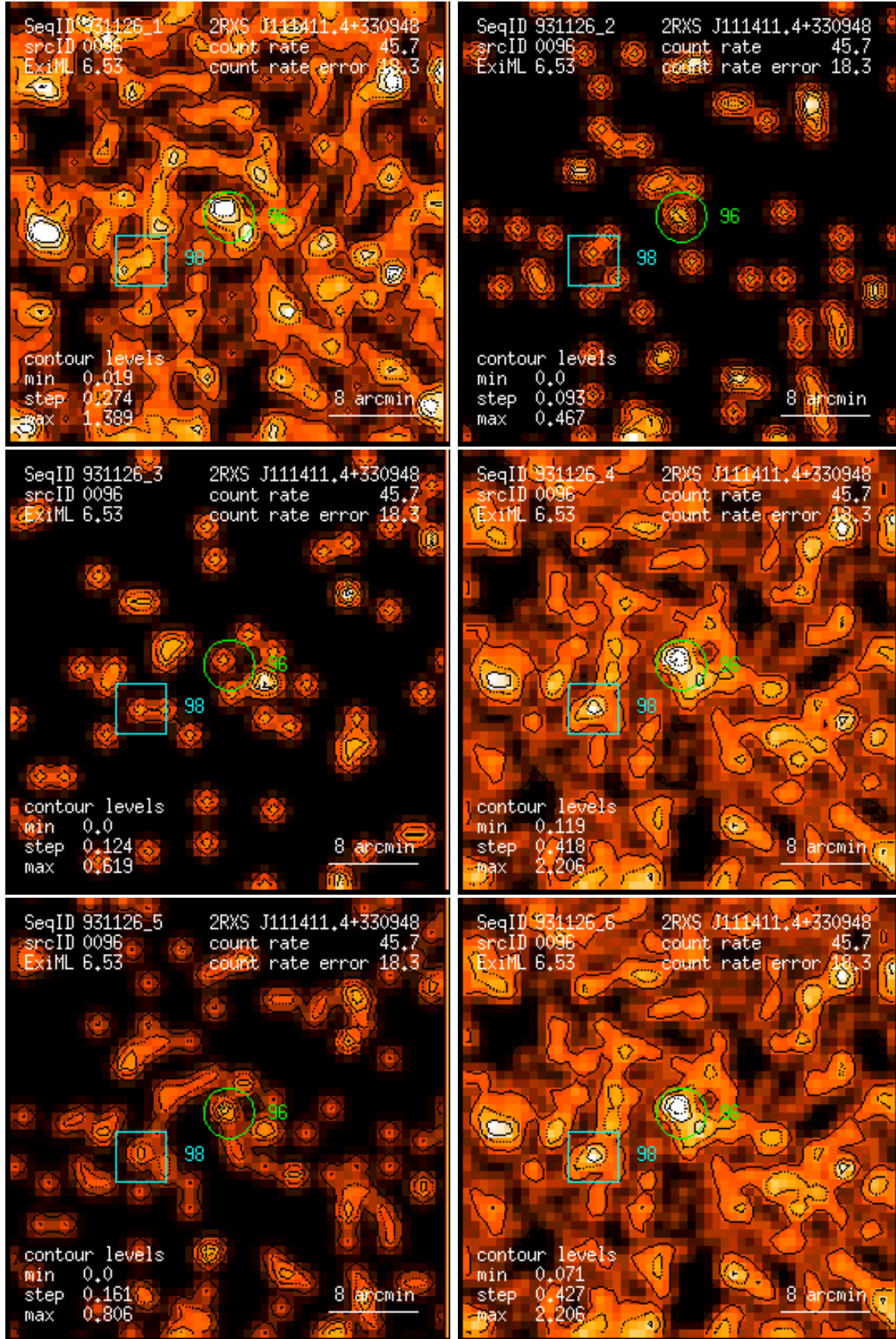
Figure 96: RASS 931126: detection 0096: band rate images, Gaussian filter: (1) PSPC channels 11 – 41, (2) 52 – 90, (3) 91 – 201, (4) 11 – 235, (5) 52 – 201, (6) 11 – 201. Broad band rates in counts/ks. Band rate contour levels in counts/ks/arcmin 2 .
