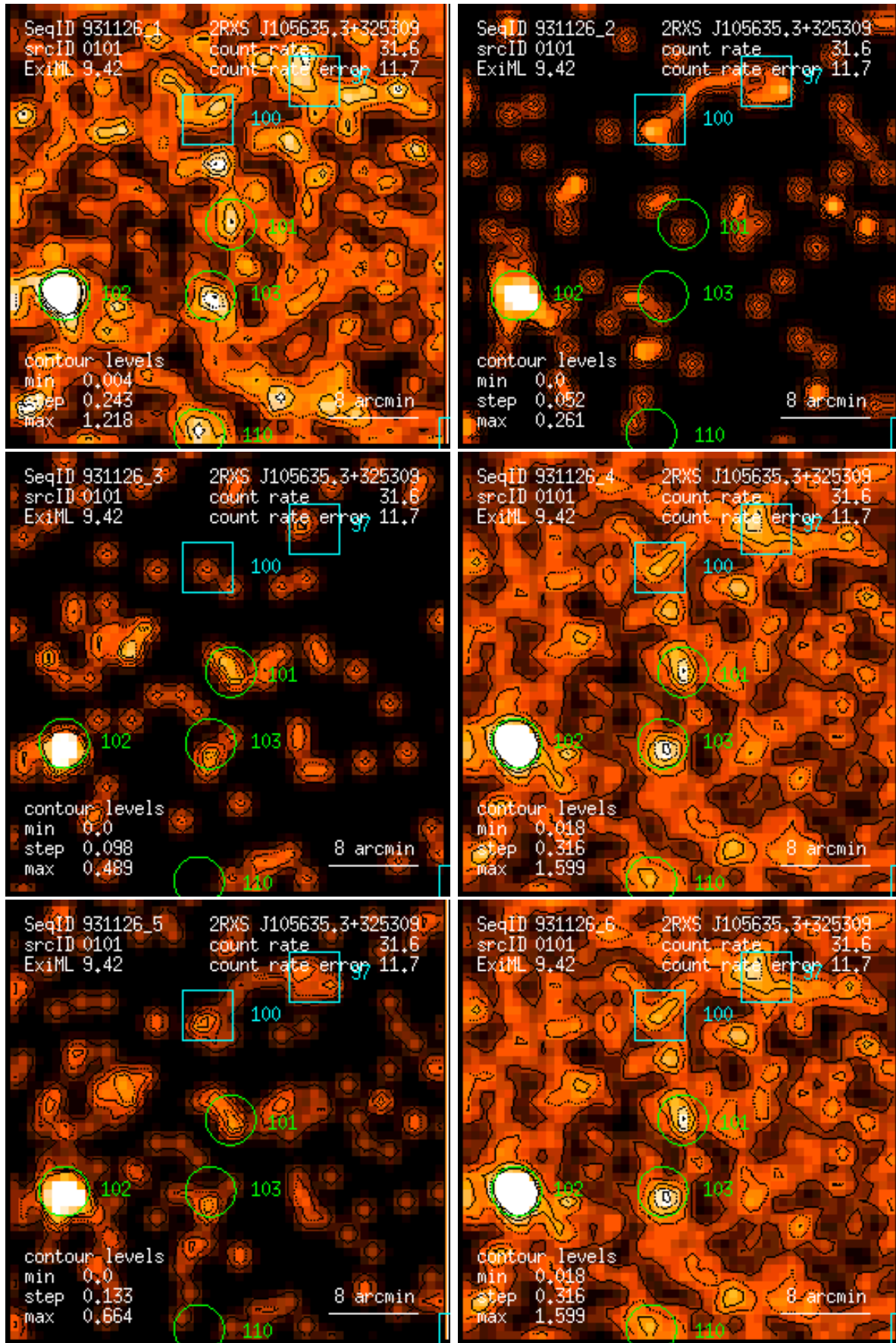
Figure 101: RASS 931126: detection 0101: band rate images, Gaussian filter: (1) PSPC channels 11 – 41, (2) 52 – 90, (3) 91 – 201, (4) 11 – 235, (5) 52 – 201, (6) 11 – 201. Broad band rates in counts/ks. Band rate contour levels in counts/ks/arcmin 2 .
