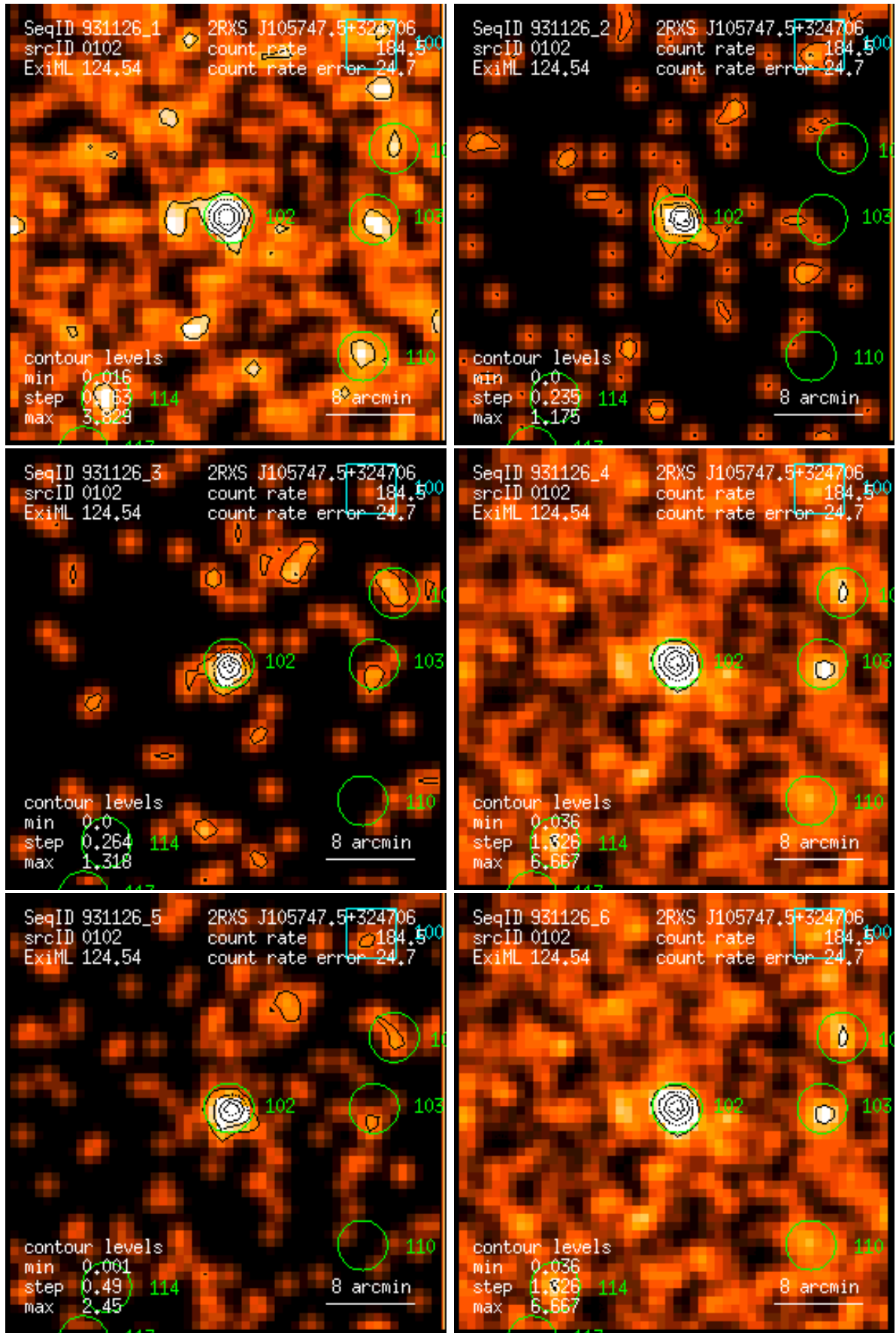
Figure 102: RASS 931126: detection 0102: band rate images, Gaussian filter: (1) PSPC channels 11 – 41, (2) 52 – 90, (3) 91 – 201, (4) 11 – 235, (5) 52 – 201, (6) 11 – 201. Broad band rates in counts/ks. Band rate contour levels in counts/ks/arcmin 2 .
