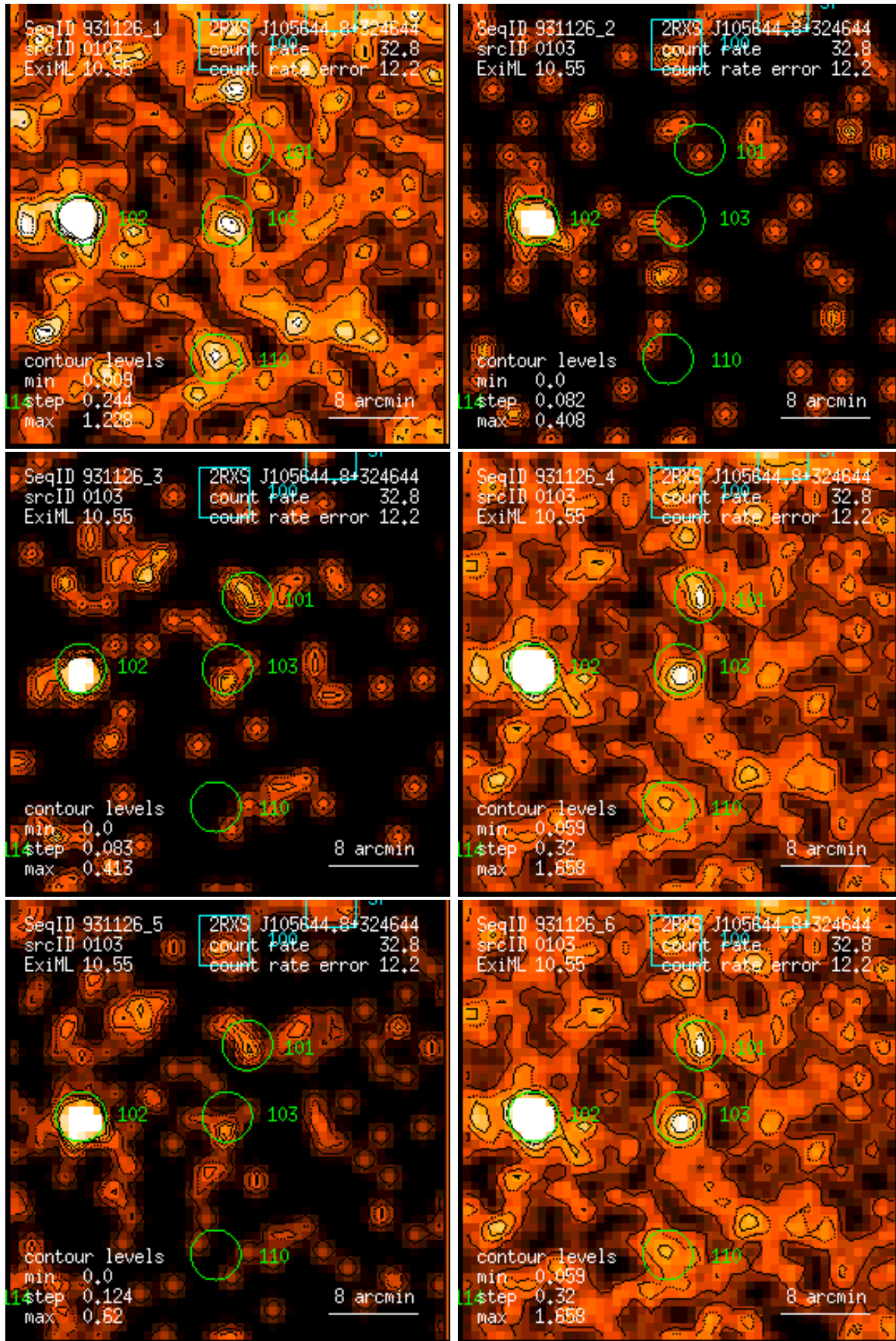
Figure 103: RASS 931126: detection 0103: band rate images, Gaussian filter: (1) PSPC channels 11 – 41, (2) 52 – 90, (3) 91 – 201, (4) 11 – 235, (5) 52 – 201, (6) 11 – 201. Broad band rates in counts/ks. Band rate contour levels in counts/ks/arcmin 2 .
